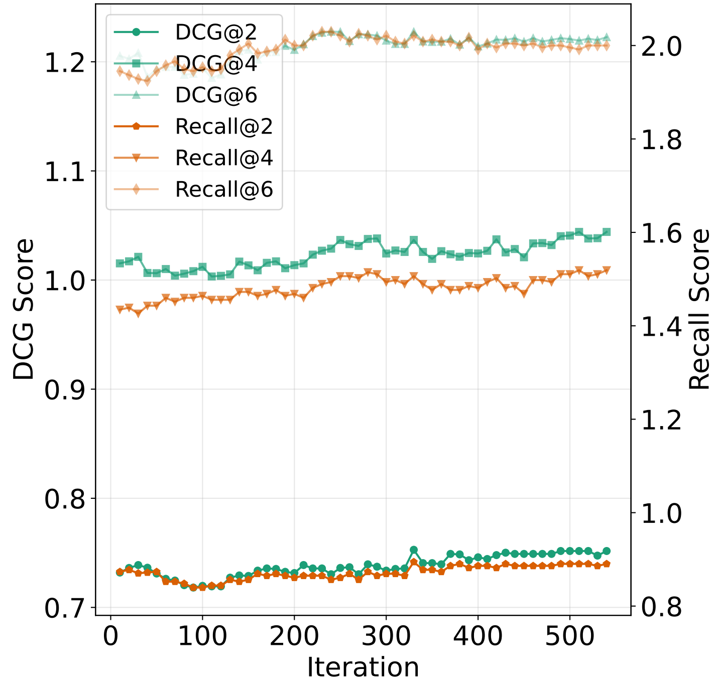
DCG and Recall Metrics
