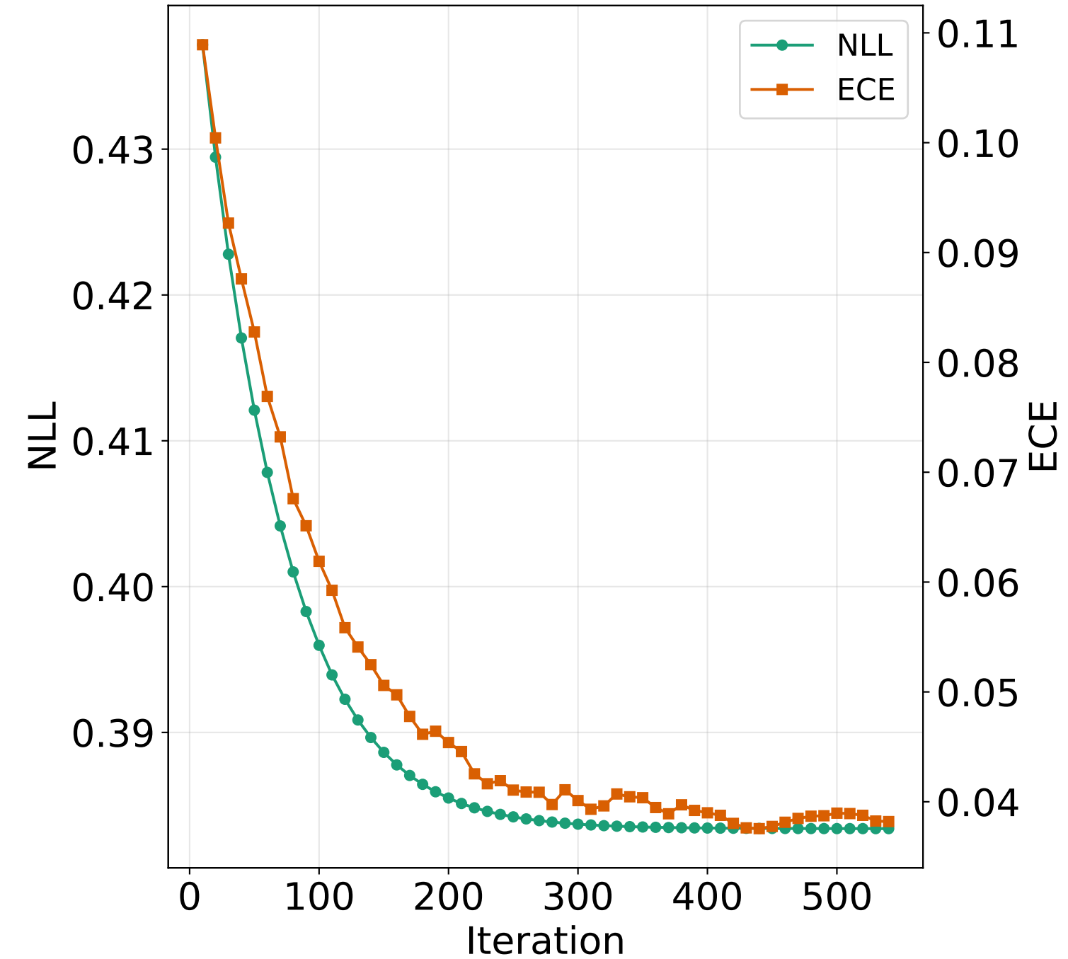
Calibration Metrics
