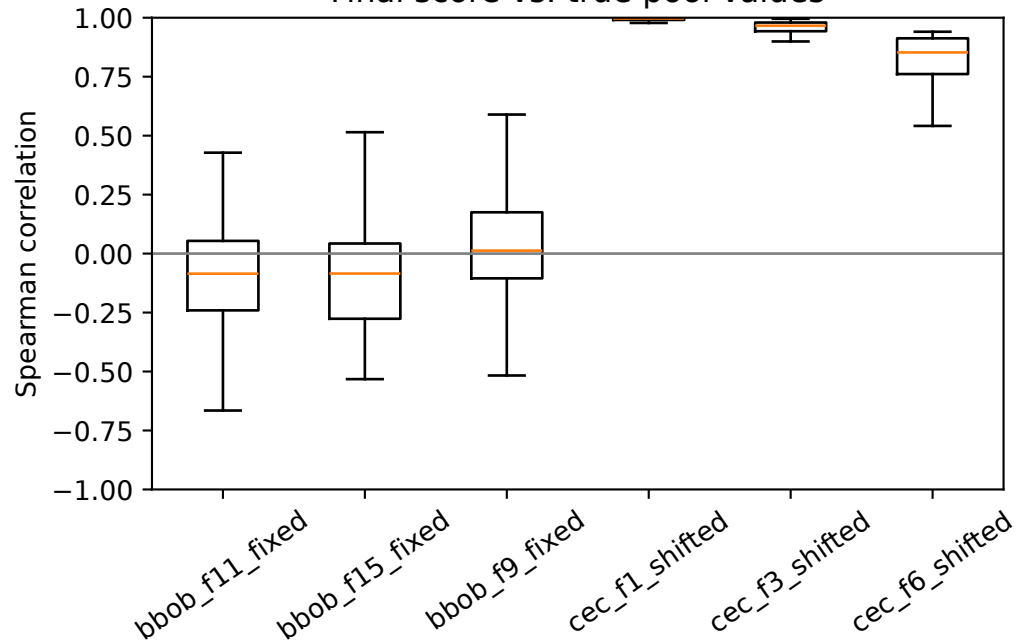
Final score vs. true pool values
