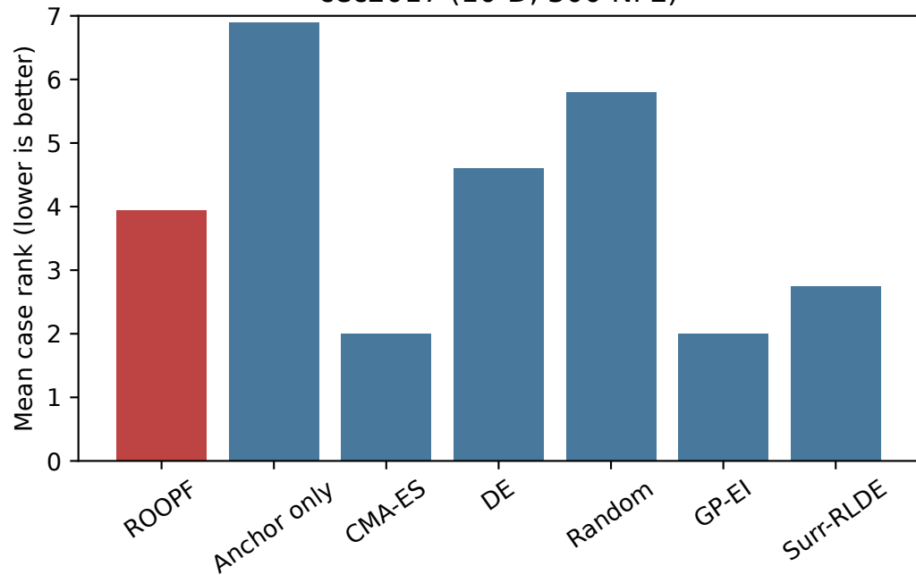
cec2017 (10-D, 300 NFE)
