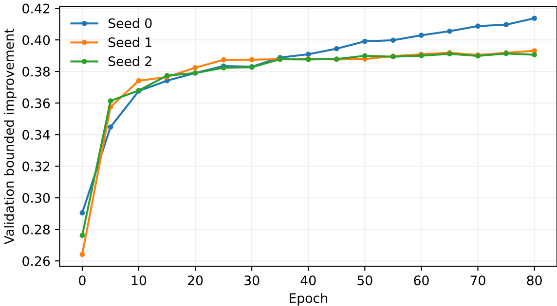
Native 20D anchor validation
