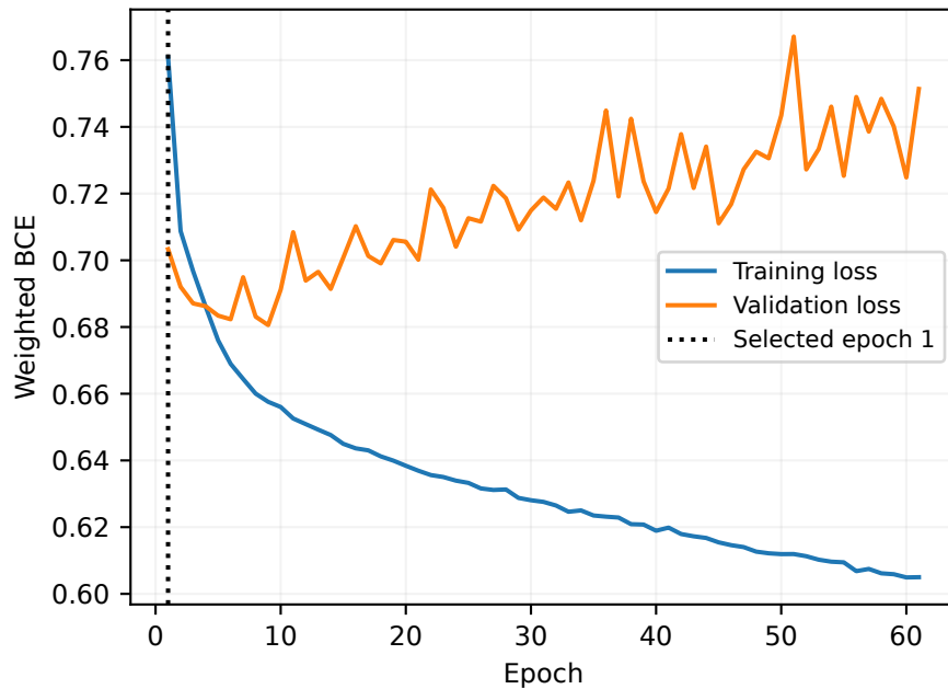
Frozen 10-D residual
