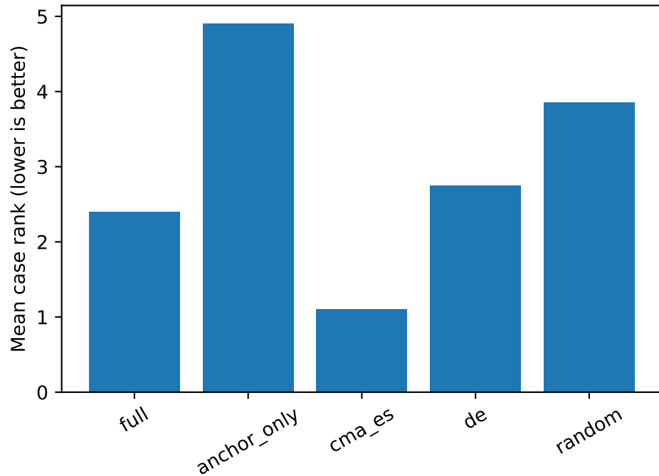
cec2017
