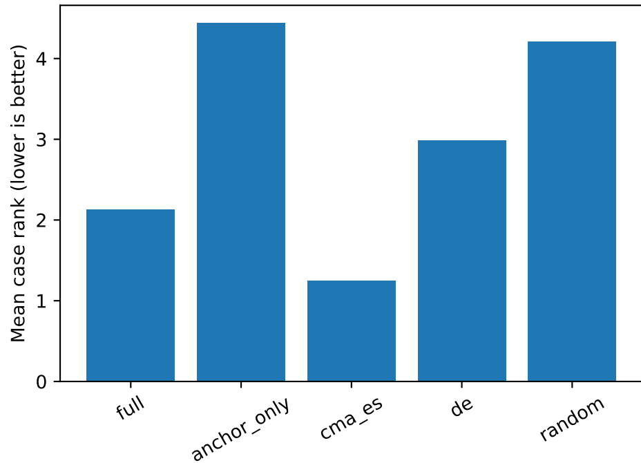
coco
