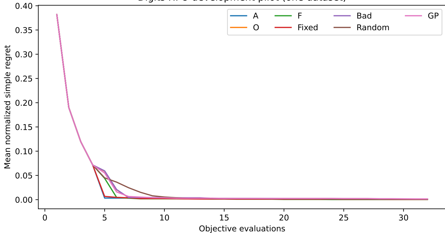
Digits HPO development pilot (one dataset)
