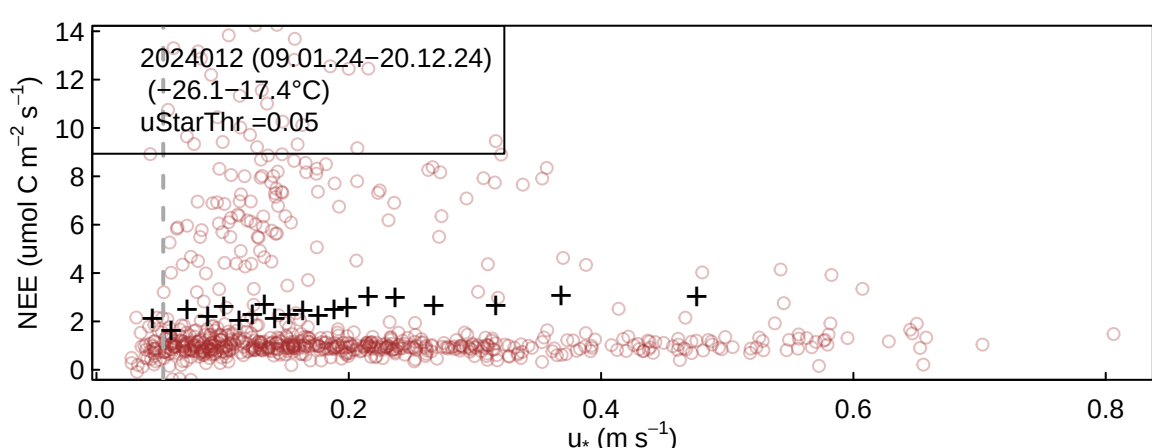
NEE versus u_{\text{Star}} for season 2024012 at Itar2024: NEE ( \mu\text{mol}+1\text{s}-1\text{m}-2 )
