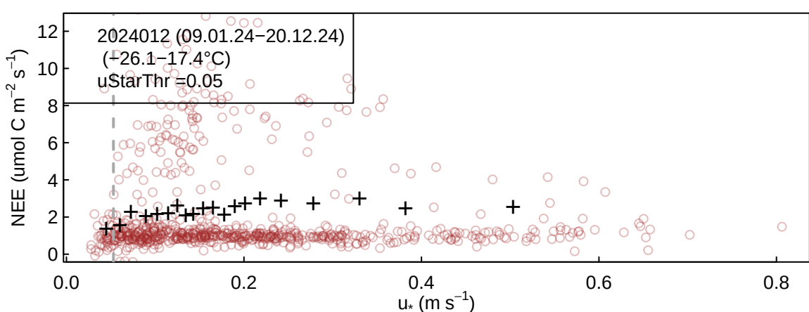
NEE versus u_{\text{Star}} for season 2024012 at Itar24: NEE ( \mu\text{mol}+1\text{s}-1\text{m}-2 )
