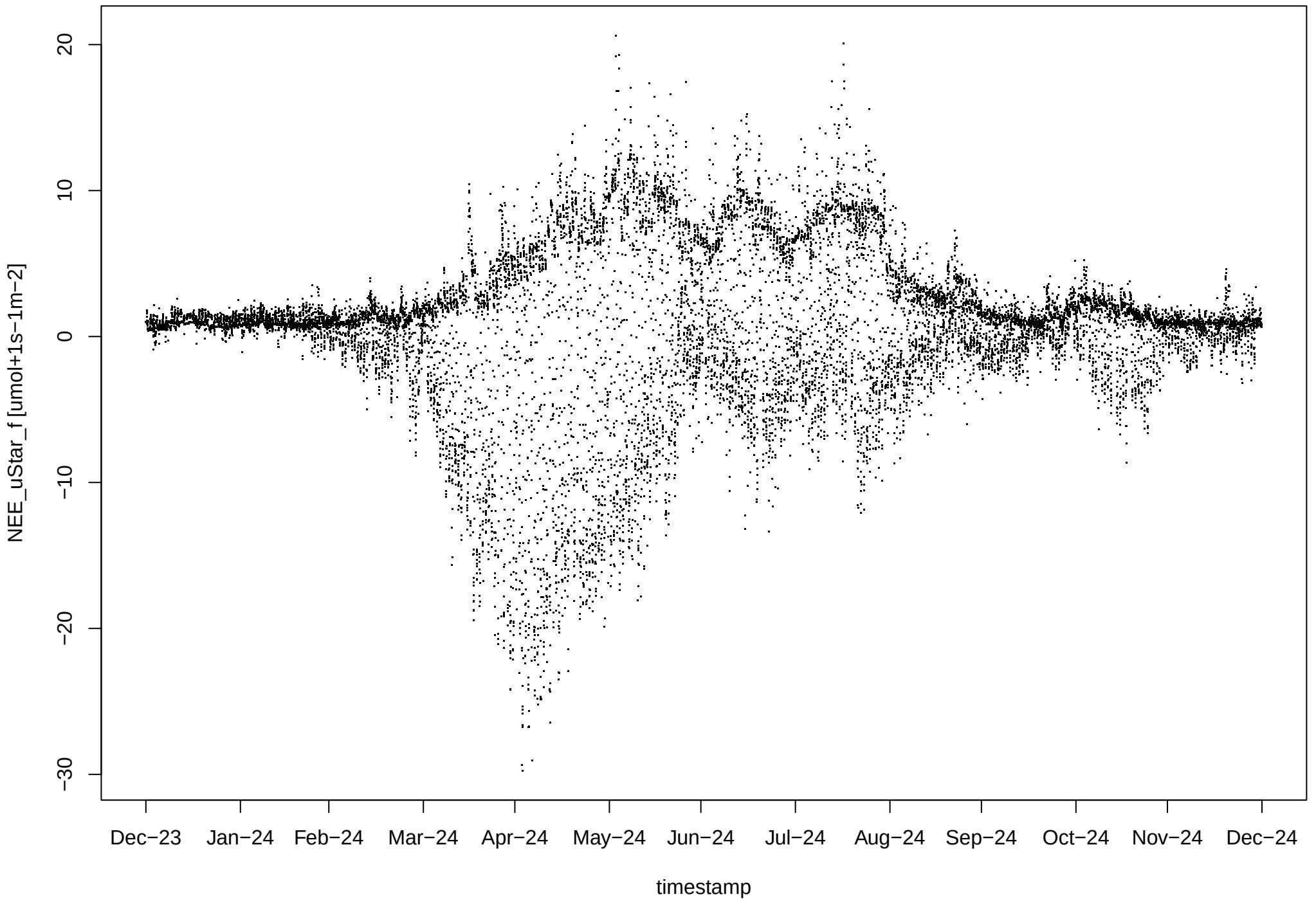
NEE_uStar_f
