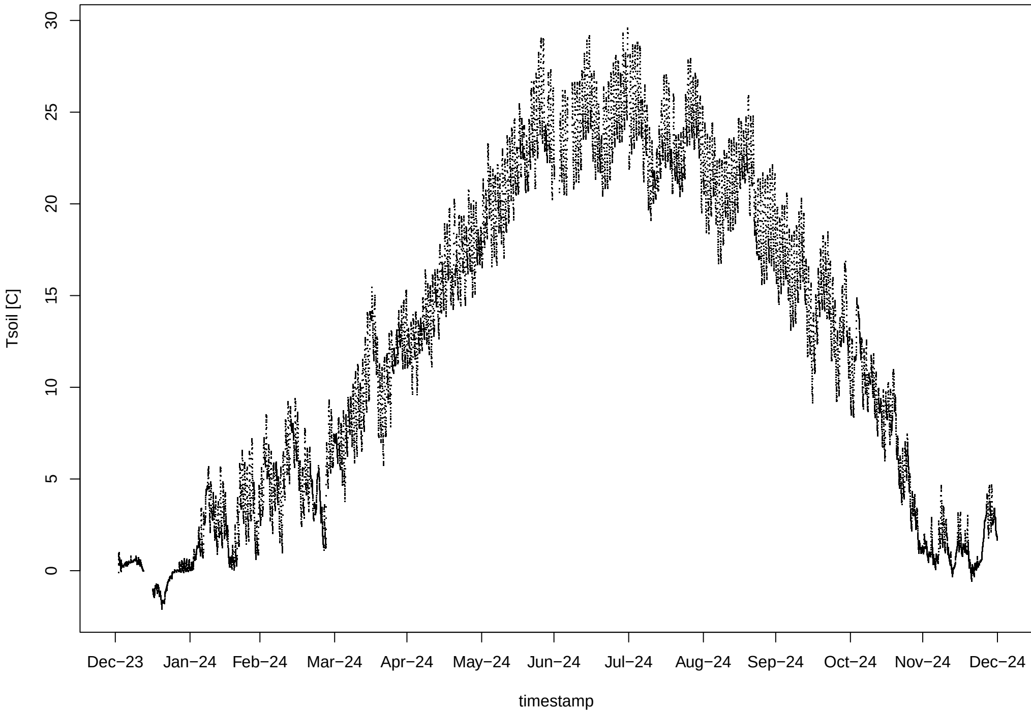
Tsoil
