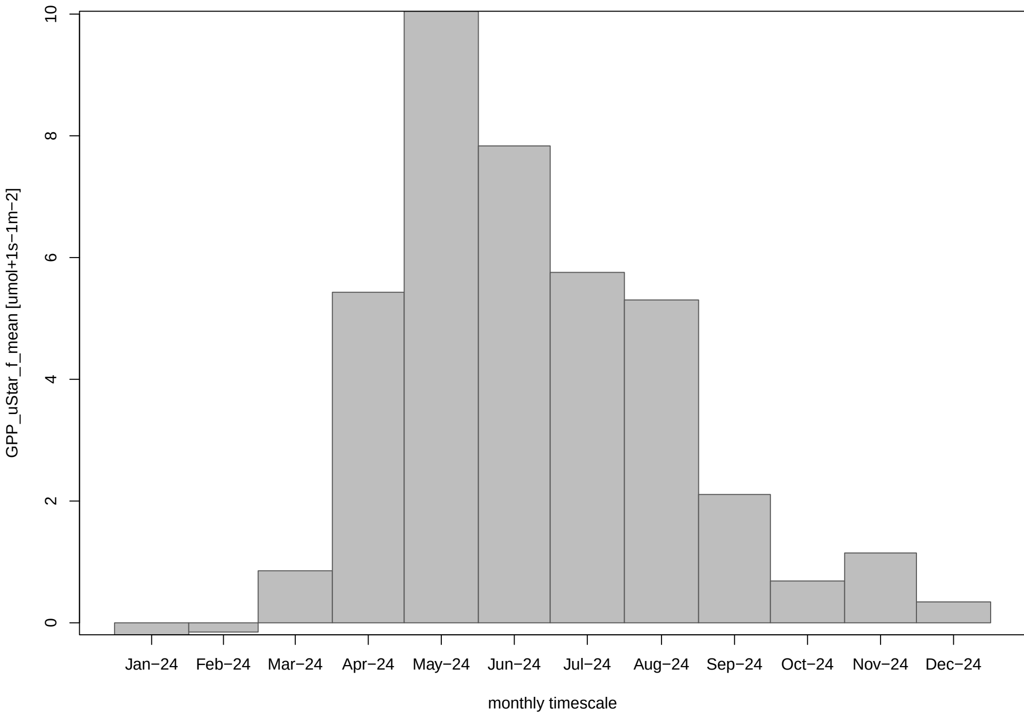
GPP_uStar_f_mean
