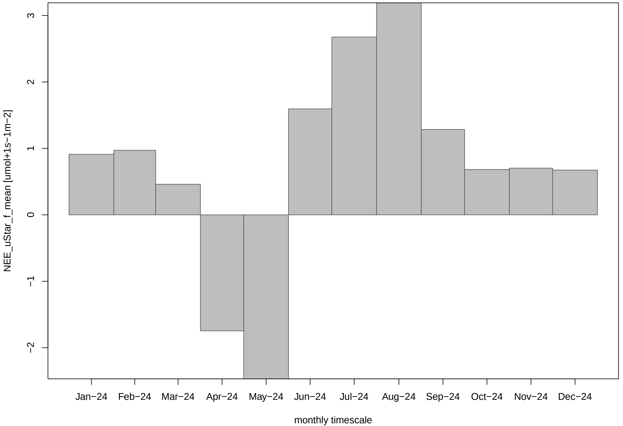
NEE_uStar_f_mean
