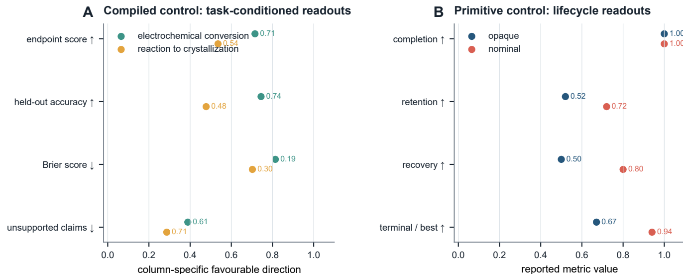
Figure 6. Experimental agency is resolved as a profile of separate readouts. A , Opaque-arm compiled-control profiles for two task families. For lower-is-better measures, horizontal position is transformed to the favourable direction while labels retain raw values. B , Primitive-control lifecycle summaries by information arm across five development worlds. Dots are not connected and no cross-metric composite is computed.
