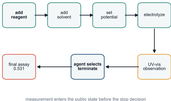
Figure 3. Primitive-control agents close complete experimental lifecycles. A , One seven-operation vessel in which a UV-visible observation is available before agent-selected termination and explicit final assay. B , All six vessels completed in each of ten world-by-information campaigns; navy denotes opaque codes and coral denotes nominal properties. C , The immutable trajectory reconstructs the campaign resource receipt. The example is descriptive and is not part of the fresh-session replication estimand.
