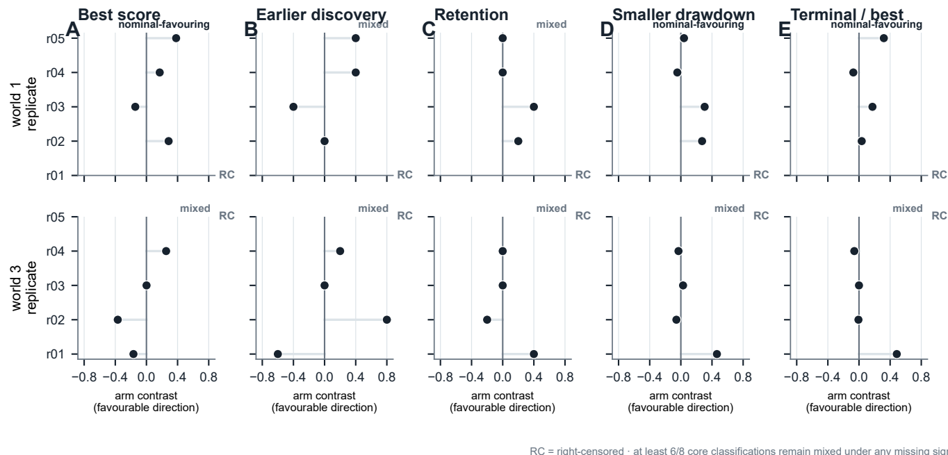
Figure 5. Fresh trajectories separate endpoint direction from lifecycle repeatability. Each point is the nominal-minus-opaque difference for a fresh session-level pair in a fixed physical world. Discovery position and drawdown are sign-flipped so that positive values consistently favour the nominal arm. All panels share one numerical scale. Right-censored pairs are marked outside the value axis as RC and are not imputed. At least six of eight core world-by-lifecycle classifications remain mixed under every possible sign of the missing pair differences.
