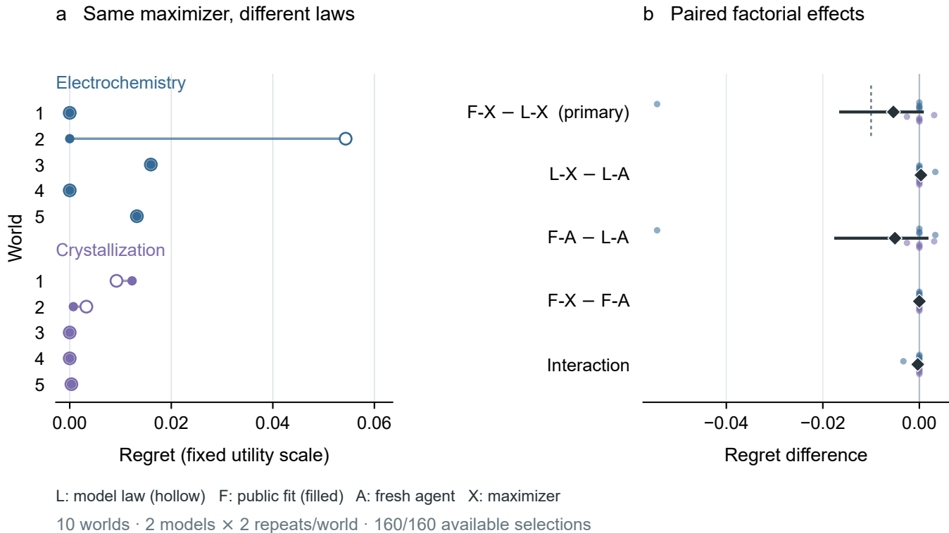
Figure 7. Fixed-evidence intervention did not establish a material repair benefit. a , Every world has its own row. Hollow and filled points show model-law and fitted-law regret under the same maximizer, averaged over two models and two repeats; concentric points denote equality. Blue denotes electrochemistry and purple crystallization. b , Colored points are individual world effects; black diamonds and lines show means and prespecified intervals (95% primary; 98.75% secondary). The dotted primary reference is -0.01. Interaction is (R_{F-X} - R_{L-X}) - (R_{F-A} - R_{L-A}) in regret. Zero-width intervals describe observed equality, not population equivalence. All 160 selections were available; repeats do not increase the ten-world denominator.
