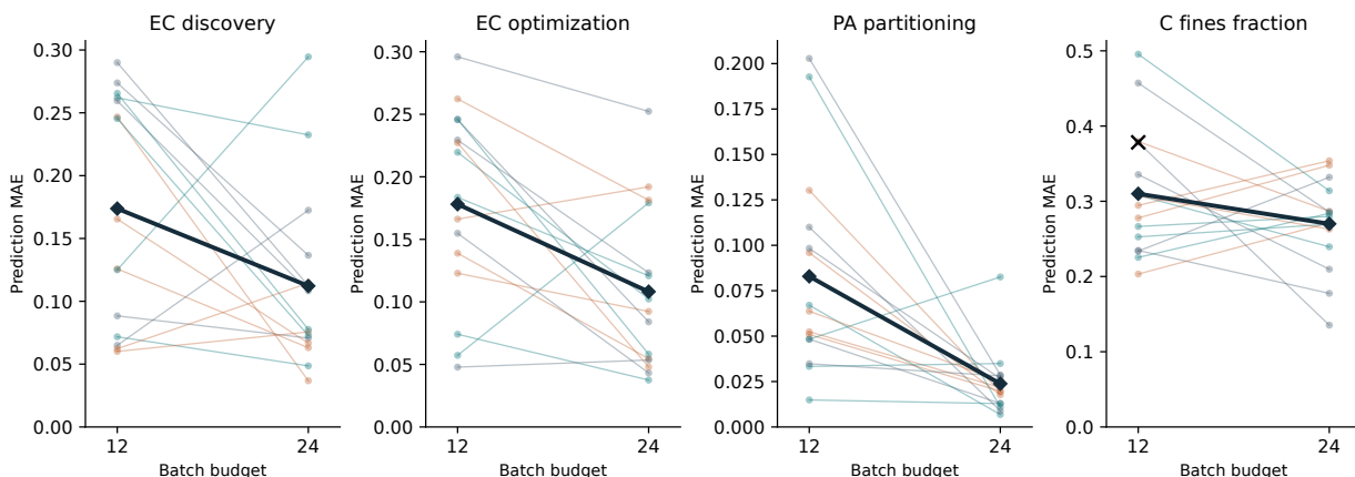
Figure 4: Budget contrasts. Thin lines connect the same world and arm across independent 12- and 24-batch sessions; dark diamonds show means. Colors follow Figure 2. The cross marks C’s source shortfall. EC panels predict score, PA predicts organic fraction, and C predicts fines fraction; vertical scales differ.
