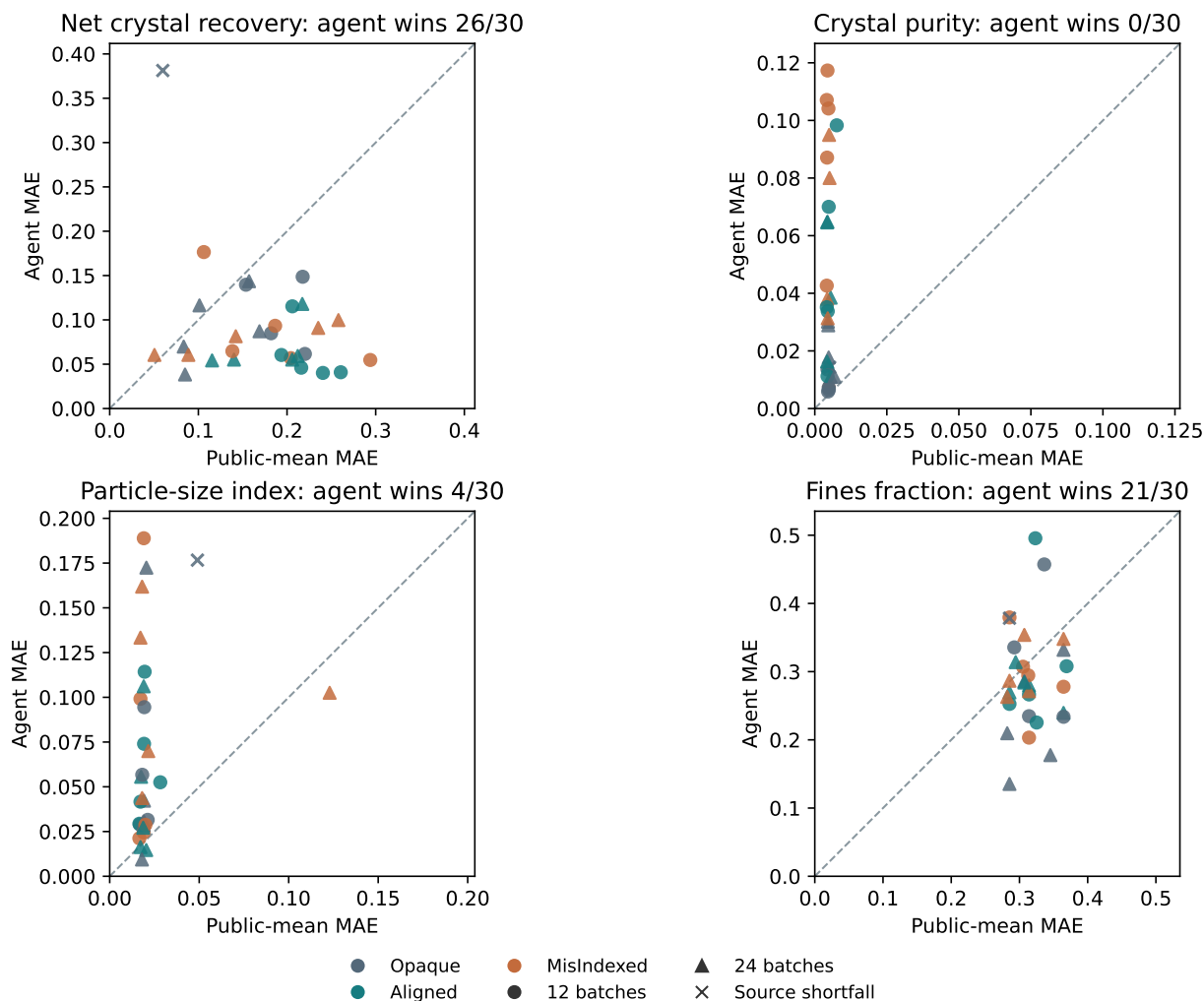
Figure 5: Same-source empirical references reveal response-specific failures in crystallization. Each panel compares agent MAE with the mean of its own public final observations for all thirty campaigns. Points above the diagonal favor the public mean. Colors denote prior arms; circles and triangles denote 12 and 24 batches. The cross marks the eleven-assay source. Panels have different scales and reuse five worlds.
