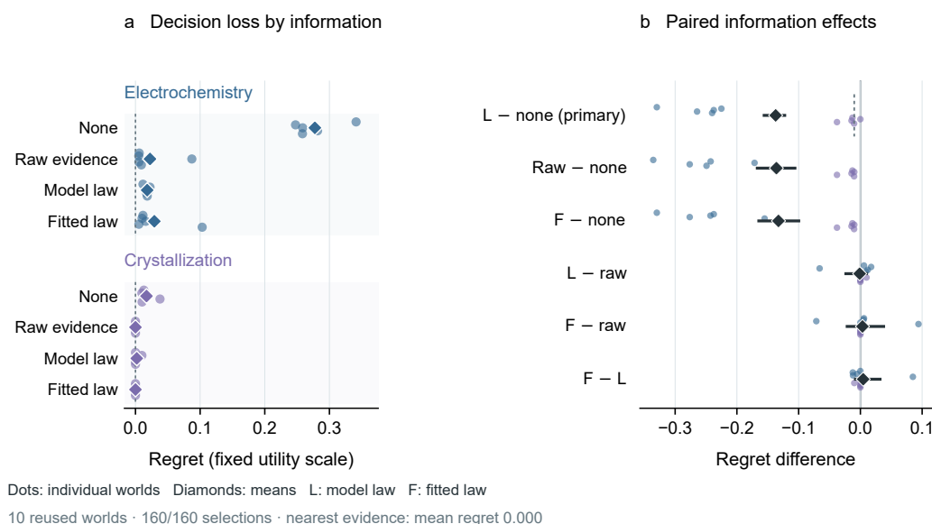
Figure 5: Artifacts support fresh decisions, while retrieval remains a strong baseline. a , Dots show world means over two models and two repeats per information condition; diamonds show task means. All 160 selections are available. Nearest evidence has zero regret in all ten worlds. b , Colored points show paired world effects; black diamonds and lines show means and prespecified intervals (95% primary; 99% for five secondary comparisons). The dotted primary reference is -0.01. L/F denote model-generated/fitted laws supplied without raw observations. These are new candidate plans in the ten reused worlds, not new physical mechanisms or additional independent replication worlds.
