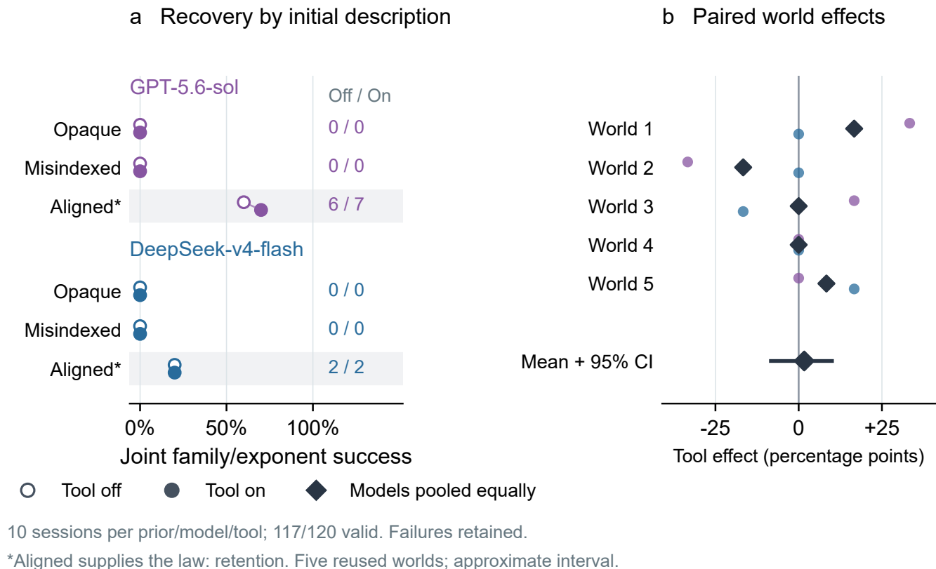
Figure 5. Valid submissions and optional numerics do not ensure structural recovery. a , Joint family/exponent success by prior, model and tool availability; each point retains ten scheduled sessions. All successes are in the aligned-prior stratum, where the correct law was supplied. b , Paired effects in five reused worlds and the equally weighted mean with its prespecified approximate 95% interval. Tool availability is the intervention: GPT used it in 0/30 sessions and DeepSeek in 20/30. Three failures remain in the denominator.
