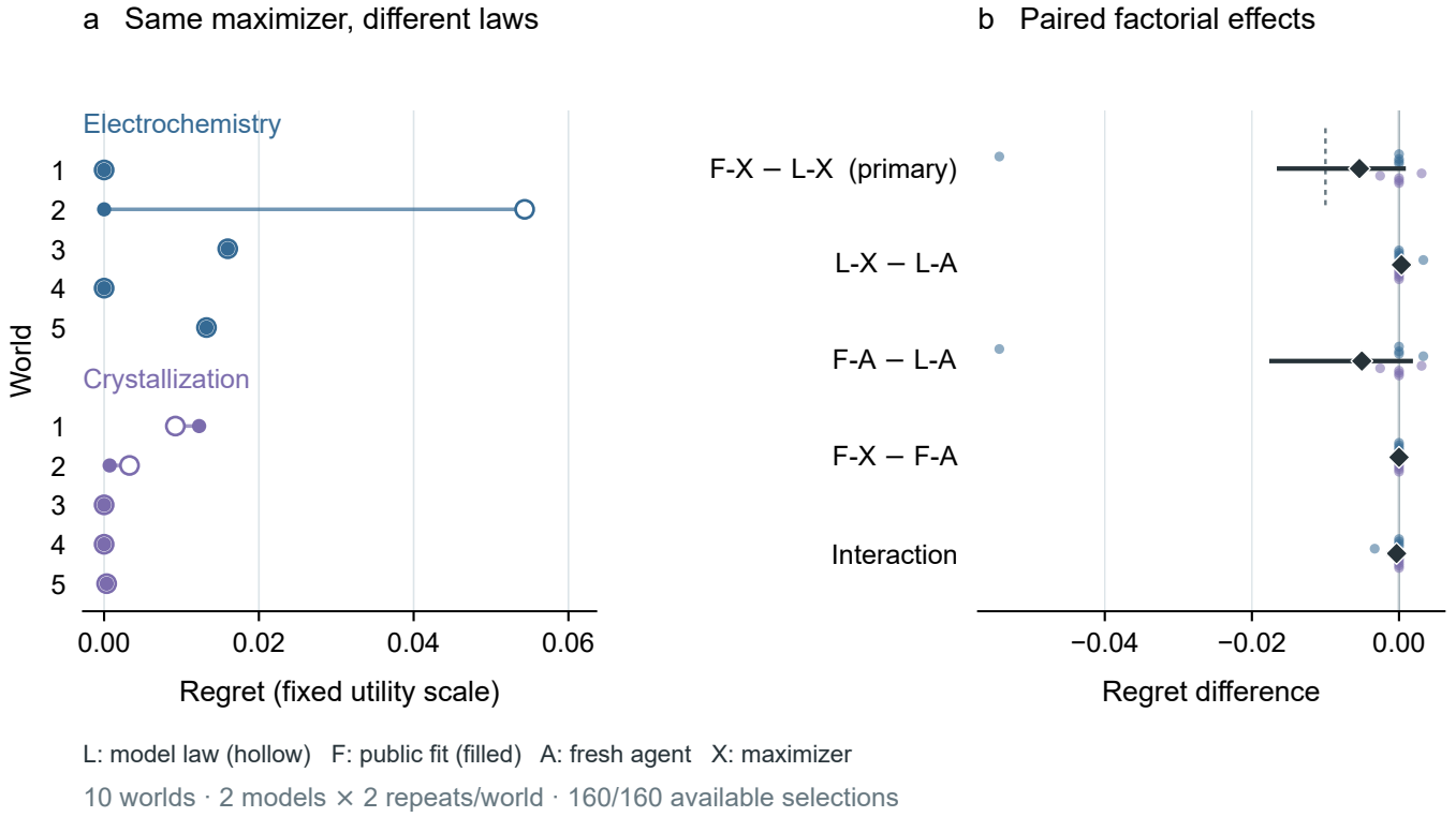
Figure 8. Fixed-evidence intervention did not establish a material repair benefit. a , Every world has its own row. Hollow and filled points show model-law and fitted-law regret under the same maximizer, averaged over two models and two repeats; concentric points denote equality. Blue denotes electrochemistry and purple crystallization. b , Colored points are individual world effects; black diamonds and lines show means and prespecified intervals (95% primary; 98.75% secondary). The dotted primary reference is -0.01. Interaction is (R_{F-X} - R_{L-X}) - (R_{F-A} - R_{L-A}) in regret. Zero-width intervals describe observed equality, not population equivalence. All 160 selections were available; repeats do not increase the ten-world denominator.
