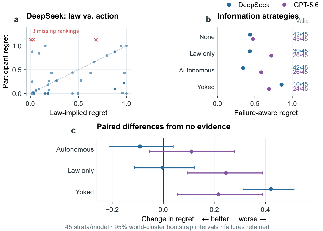
Figure 7. Law quality and information strategies have distinct decision readouts. a , Law-implied versus participant regret in the 45-cell DeepSeek matrix; 42 observed choices are dots and three missing rankings are crosses above the plotting range. The diagonal marks equal regret. b , Failure-aware strategy means with valid/scheduled counts. c , Paired strategy-minus-no-evidence differences with task-stratified world-cluster bootstrap 95% intervals, retaining all 45 strata per model. Both autonomous contrasts cross zero. The strategy block is development evidence; yoked failures prevent a pure acquisition-effect interpretation. Complete-ranking diagnostics remain in the appendix.
