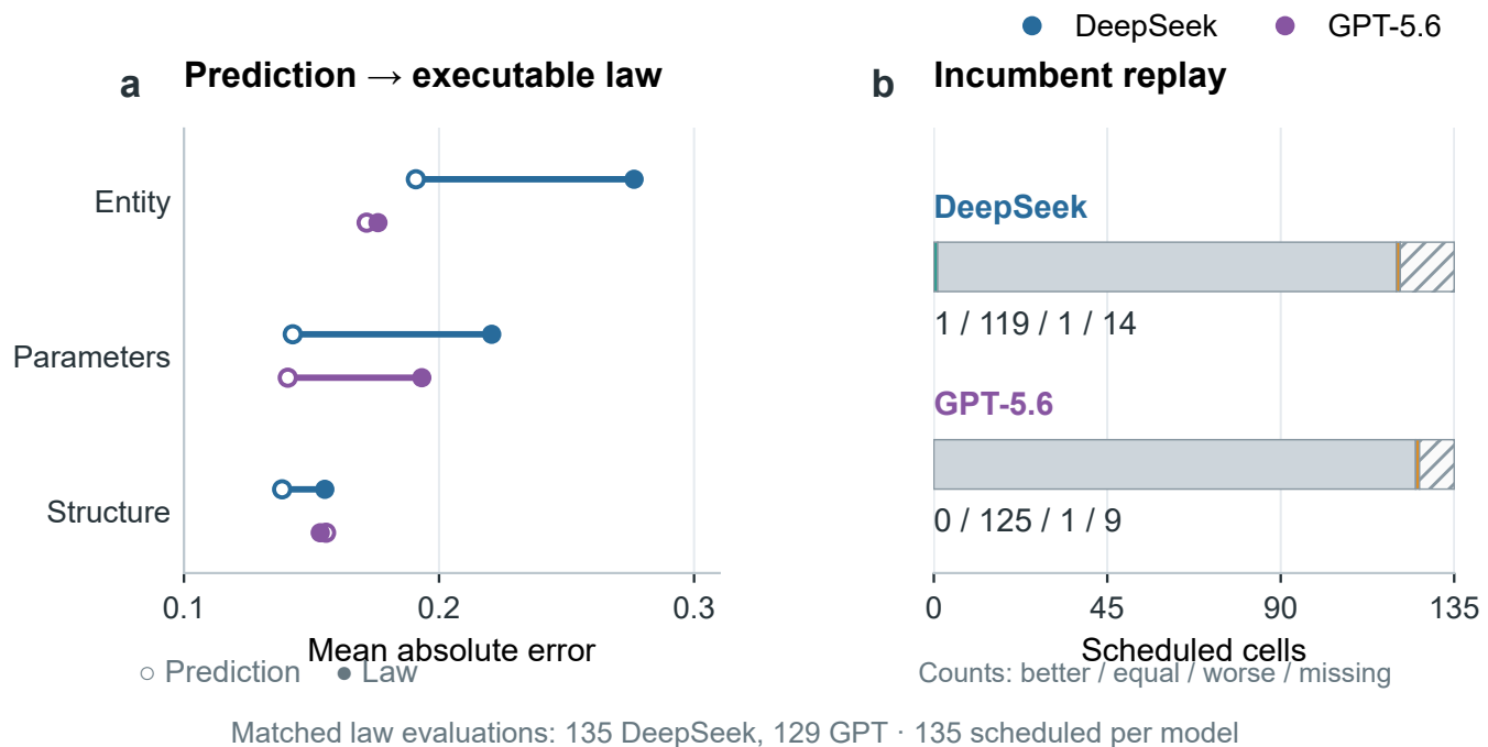
Figure 6. Lower executable-law error coexists with near-zero incumbent gain. a , Hollow and filled points show final-prediction and executable-law MAE on the same law-evaluable cells, grouped by locus and model; connecting lines show compression differences, not uncertainty. The matched denominators are 135 DeepSeek and 129 GPT laws. b , Better/equivalent/worse/unavailable incumbent-replay counts retain all 135 scheduled cells per model; hatching marks unavailable readouts. These are descriptive configuration contrasts and incumbent replays, not causal artifact effects or unseen-action benefits.
