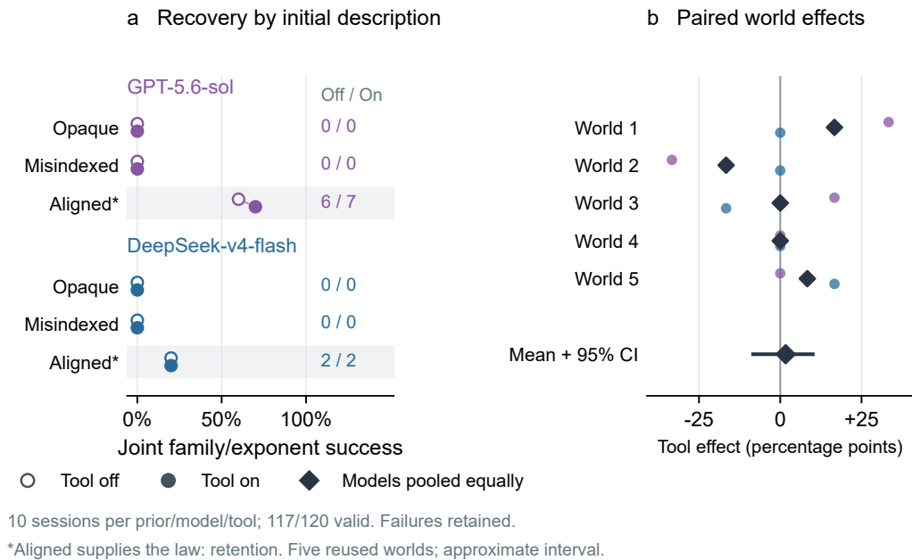
Figure 3: Valid submissions and optional numerics do not ensure structural recovery. a , Joint family/exponent success by prior, model and tool availability; each point retains ten scheduled sessions. All successes are in the aligned-prior stratum, where the correct law was supplied. b , Paired effects in five reused worlds and the equally weighted mean with its prespecified approximate 95% interval. Tool availability is the intervention: GPT used it in 0/30 sessions and DeepSeek in 20/30. Three failures remain in the denominator.
