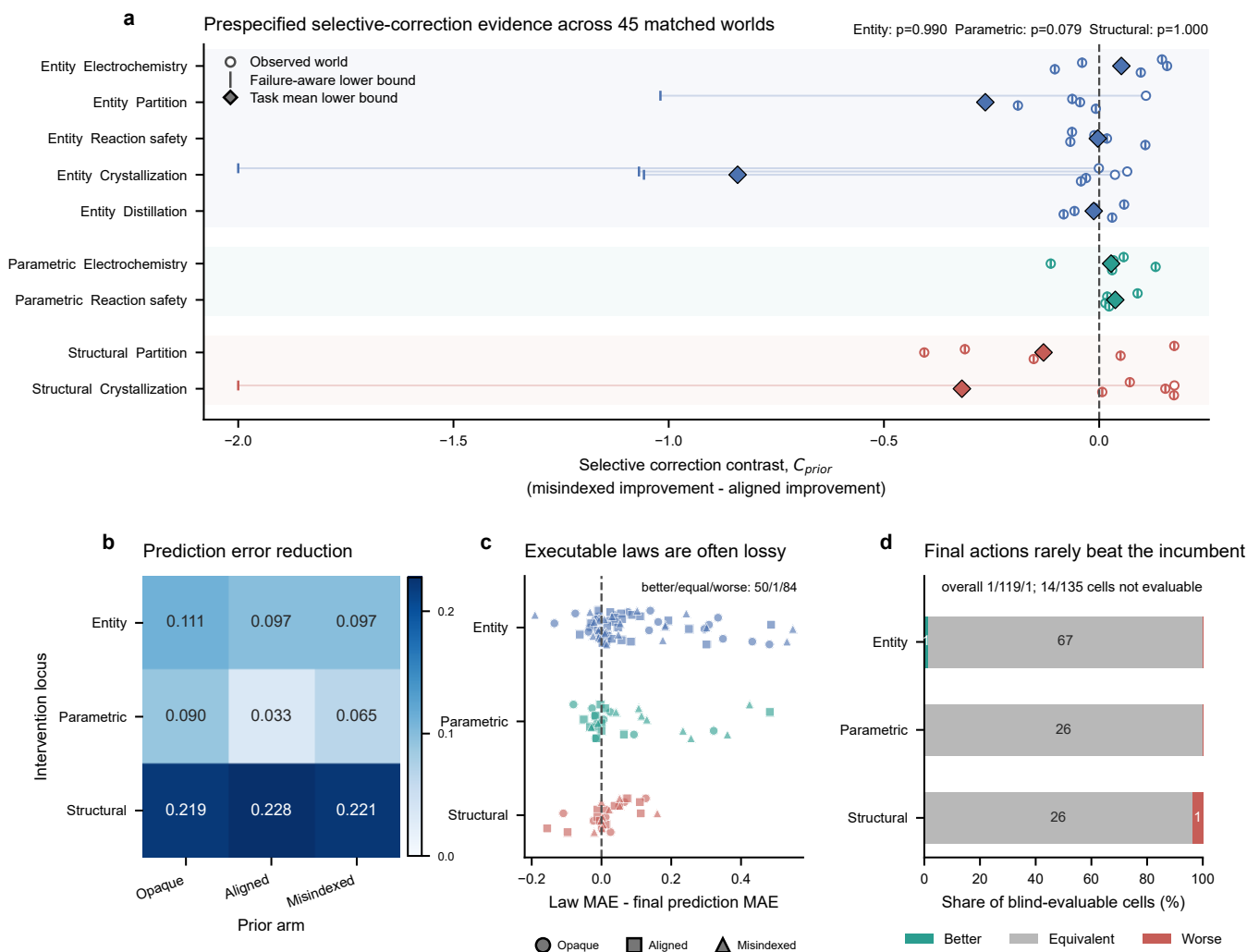
Figure 5. Predictive learning, selective correction, executable-law compression and incumbent replay dissociate.
