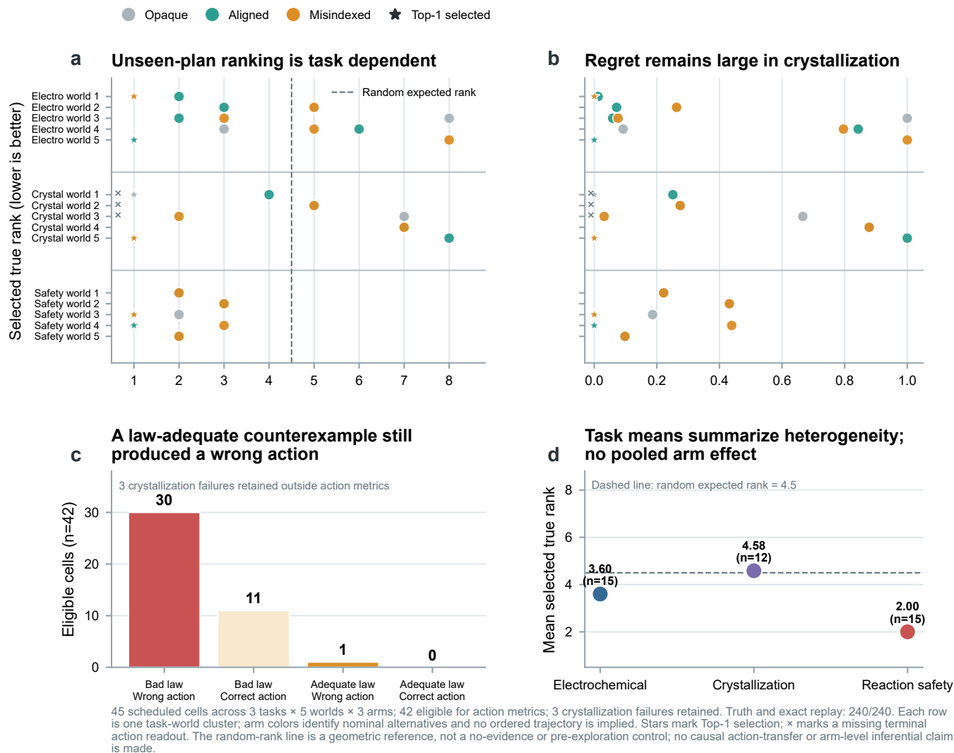
Figure 6. Terminal selection of unseen plans is partial and task dependent. a , Selected true rank for every eligible cell; rows group task-world clusters, arm colors identify the three initial-model conditions and the dashed line marks the uniform-random rank expectation of 4.5. b , Normalized regret for the same cells. c , Joint law-action categories among 42 eligible cells; three crystallization failures remain outside action metrics but inside the scheduled denominator. d , Task-level mean ranks show heterogeneity across chemical workflows. The random-rank line is a geometric reference rather than a no-evidence control, and no causal action-transfer or pooled arm claim is made.
