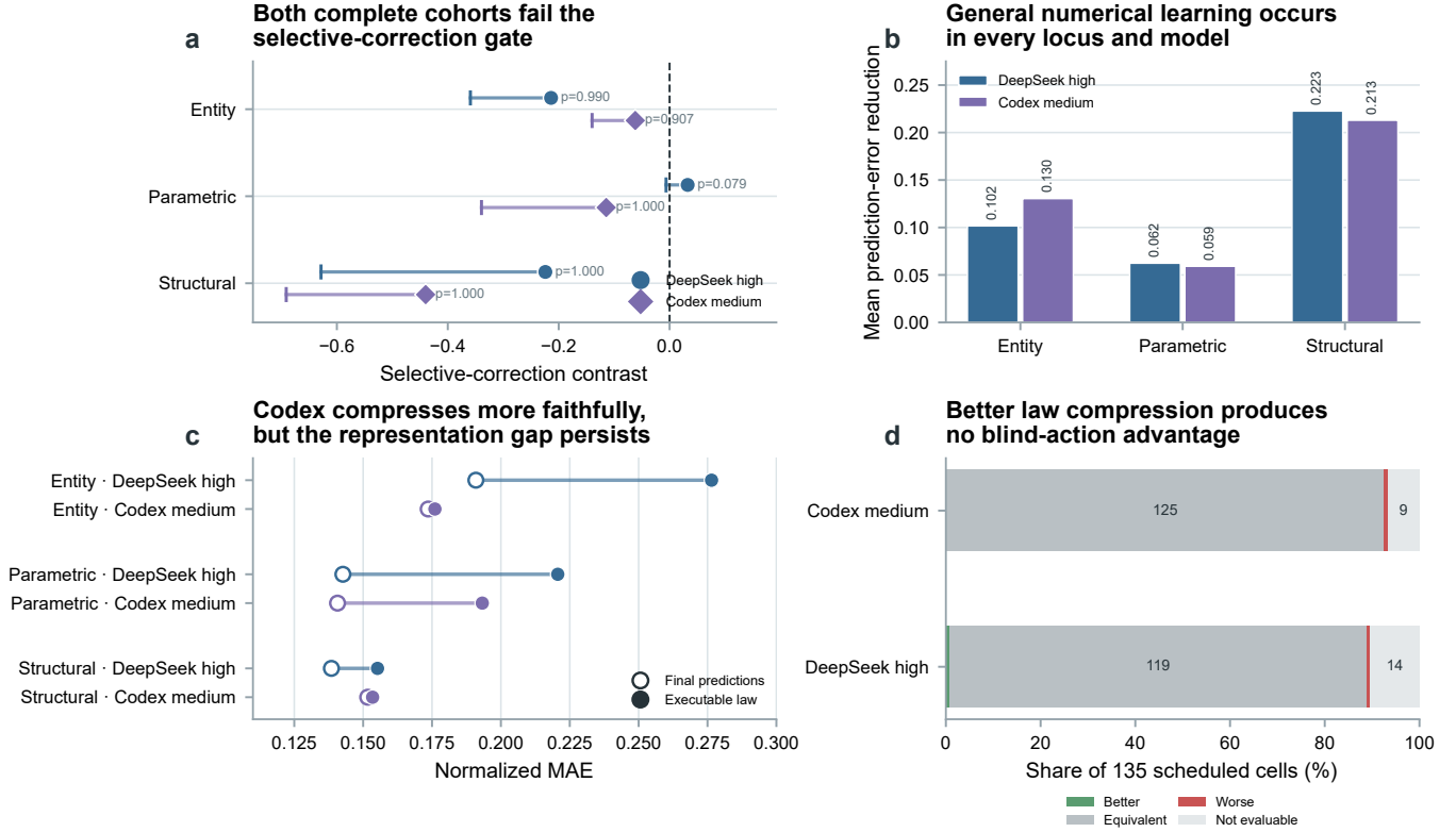
Figure 5. Better executable laws still do not produce better actions. a , Registered failure-aware selective-correction estimates and one-sided lower bounds for entity, parametric and structural loci in the complete DeepSeek and Codex C2 cohorts; both cohorts fail every locus gate. b , Mean pre-to-final prediction-error reduction by locus and model. c , Final explicit-prediction and executable-law MAE on the matched C2 surface; Codex reduces the representation gap, especially at entity and parametric loci. d , Blind better, equivalent, worse and not-evaluable outcomes over all 135 scheduled cells per model. Model differences are matched descriptive, not provider causal effects.
