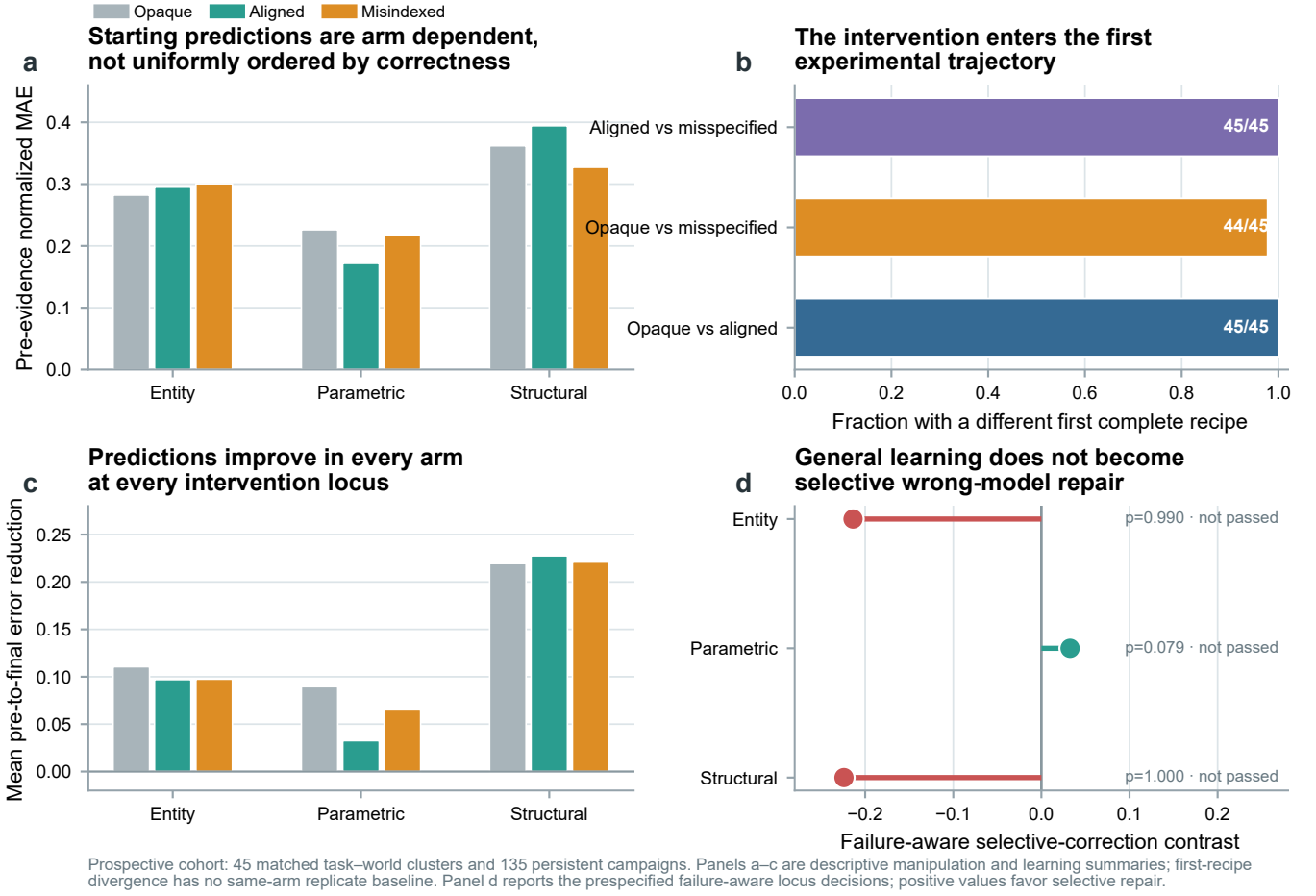
Figure 3. Initial models redirect search, but the evidence does not establish selective repair of the wrong model. a , Mean pre-evidence normalized prediction error by locus and initial-model arm; correctness does not impose a uniform starting-error ordering. b , Fraction of 45 matched task-world clusters in which the first complete experimental recipe differs between each pair of arms. This retrospective manipulation check has no repeated same-arm baseline. c , Mean pre-to-final prediction-error reduction. Every arm improves at every locus. d , Prespecified failure-aware selective-correction contrasts and locus p values. Positive values favor greater repair in the misspecified arm; no locus passed.
