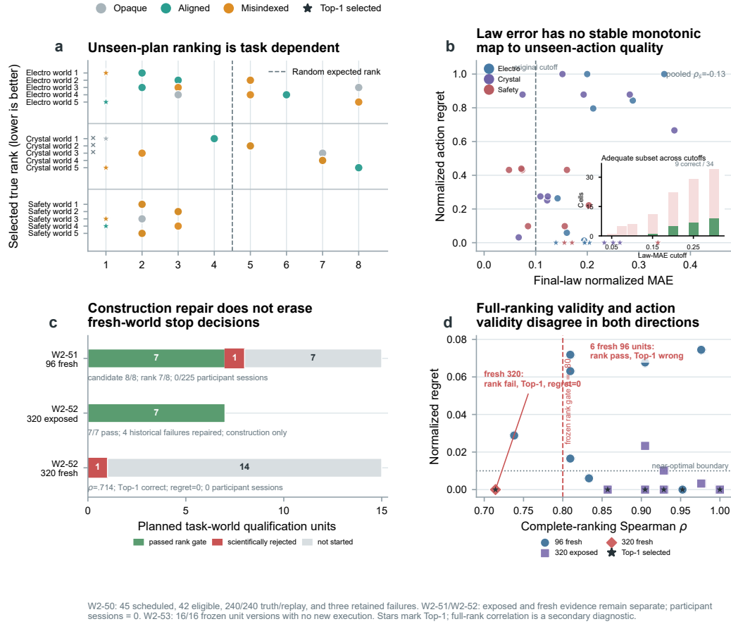
Figure 4: Agent law-action decoupling and evaluator rank-action misalignment. a , True rank for 42 eligible W2-50 cells; all 45 scheduled cells remain in the denominator. b , Continuous law error versus regret, with Top-1 stars and a seven-cutoff inset. c , Frozen W2-51/W2-52 qualification dispositions separate exposed construction from fresh qualification; participant execution is zero. d , Spearman correlation versus regret for all 16 frozen W2-53 unit versions. No panel revises a historical stop decision.
