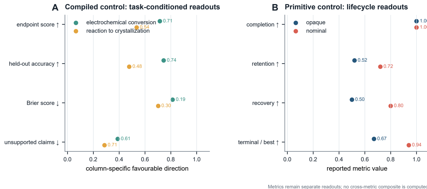
Figure 6. Experimental agency is resolved as a profile of separate readouts. A , Opaque-arm compiled-control profiles for two task families. For lower-is-better measures, horizontal position is transformed to the favourable direction while labels retain raw values. B , Primitive-control lifecycle summaries by information arm across five development worlds. Dots are not connected and no cross-metric composite is computed.
