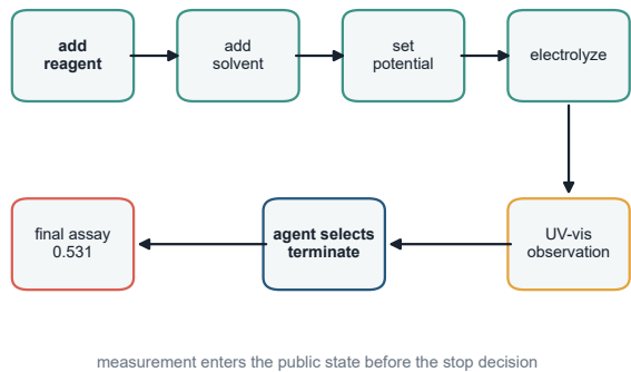
Figure 3 | Primitive-control agents close complete experimental lifecycles. The agent selects operations, observes intermediate evidence, decides when to stop and requests final assay under a reconstructable campaign ledger.
