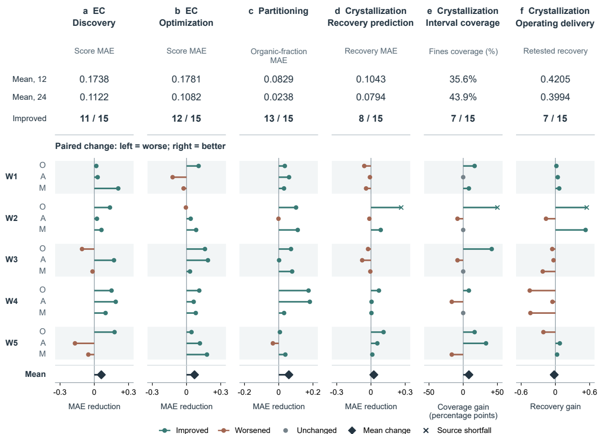
O: Opaque A: Aligned M: MisIndexed. Each column contains 15 matched pairs; world labels are system-specific. Independent sessions; 24 batches also allow more operations and computation. All C coverage values remain below the nominal 80%.
