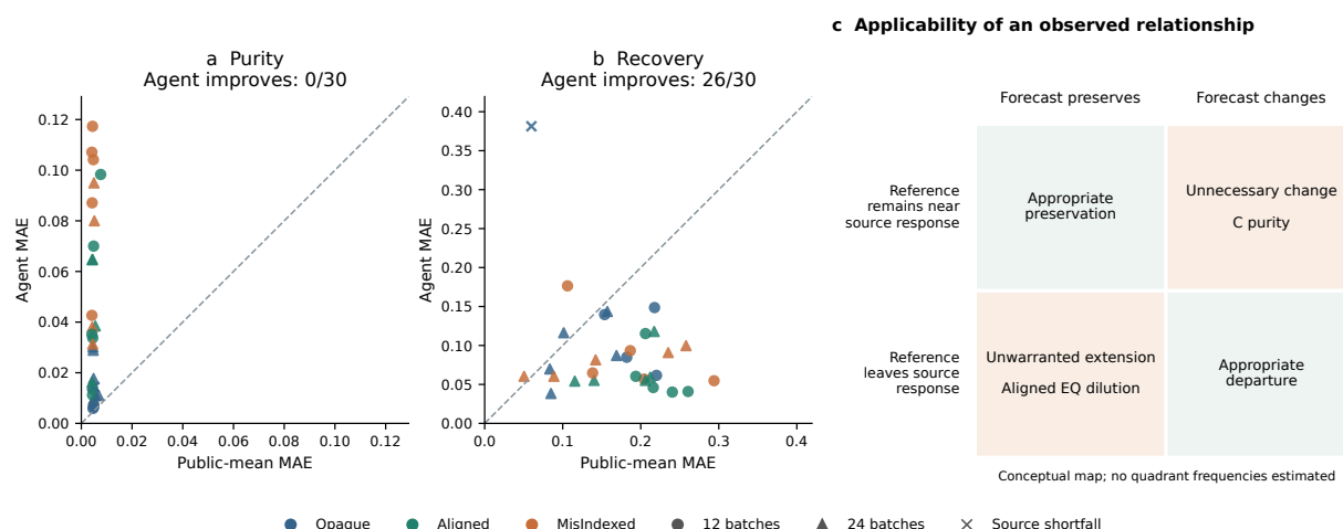
Figure 5: Preserving and revising observed relationships are distinct prediction decisions. Left: crystallization purity and recovery errors compared with the mean of each campaign's public final assays; points above the diagonal favour the mean. Agents lose on purity in all thirty campaigns and improve recovery in twenty-six. Symbols distinguish budgets and the source-assay shortfall. Right: a conceptual map places crystallization purity and aligned dilute-equilibrium predictions in complementary error categories. The map is an interpretation of these specific response patterns, not a cohort-wide classifier, measured quadrant frequency or account of internal belief updates. Stable purity is specific to the tested conditions; a constant predictor's success does not establish mechanism discovery.
