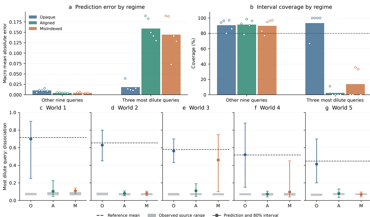
Figure 4: Regime-dependent prediction in the original autonomous equilibrium campaigns. Top: macro MAE and interval coverage for the three most dilute recipes and the other nine; small points show the five reused worlds, and the dashed line marks nominal 80% coverage. Bottom: all fifteen campaigns’ dissociation predictions and 80% intervals for the most dilute recipe, compared with the original five-observation reference mean in each world. Grey bands show the range of final-assay dissociation observed during each source campaign. Every source remains above the dilute test concentrations. The predictions retain the original research context. Query grouping is exploratory.
