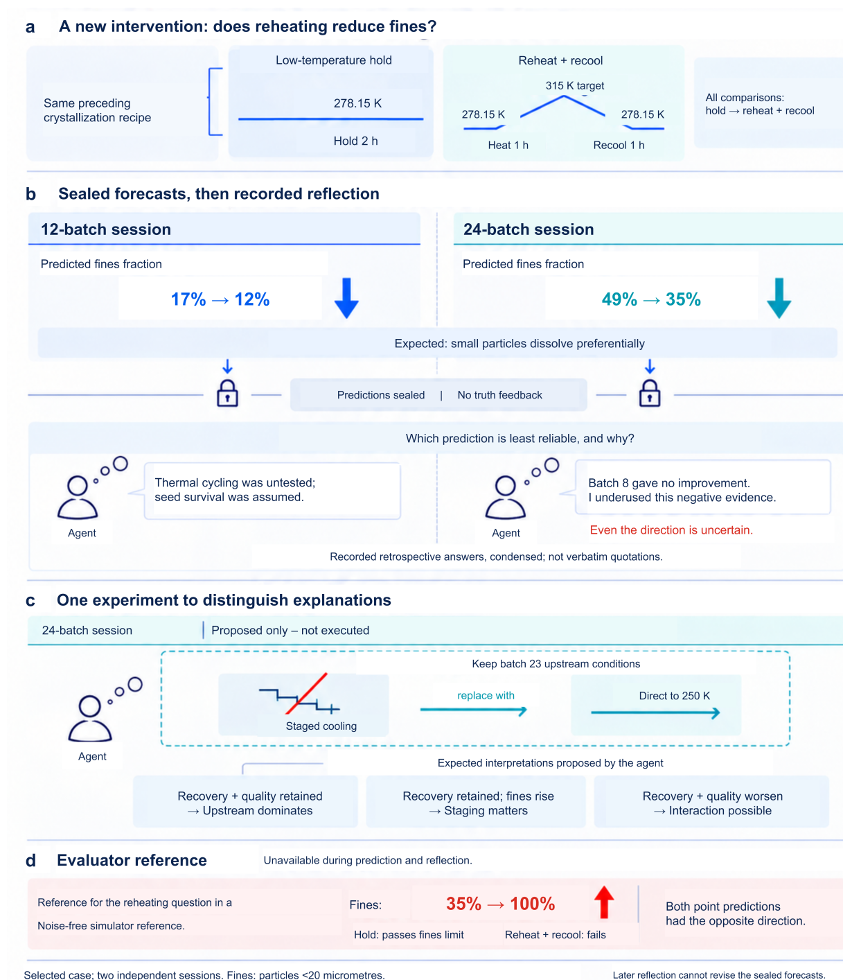
Figure 7: Sealed predictions and subsequent reflection in the same selected crystallization pair. a, The withheld comparison replaces a two-hour hold at 278.15 K with heating towards 315 K for one hour and recooling for one hour after a common preceding recipe. Thermal profiles are schematic. b, Both original sessions predict lower fines. The condensed public K2 answers follow sealed Q predictions without reference feedback. c, The 24-batch session proposes changing only the cooling procedure of its selected batch; possible outcomes would distinguish upstream, cooling and interaction explanations. This proposal was not executed. d, The evaluator's reference concerns the thermal intervention in a, not the proposed experiment in c, and was unavailable during Q and K2.
