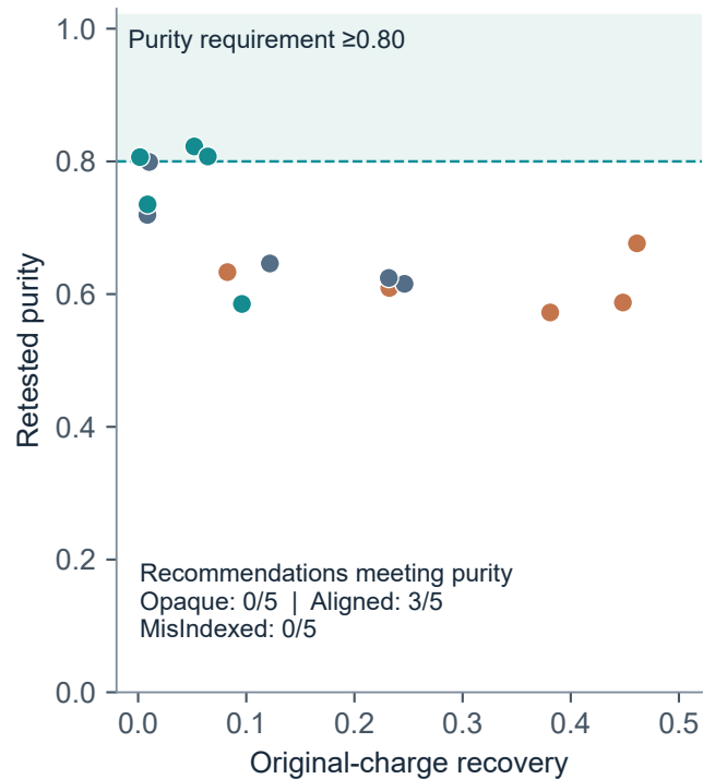
c Purification constraints
