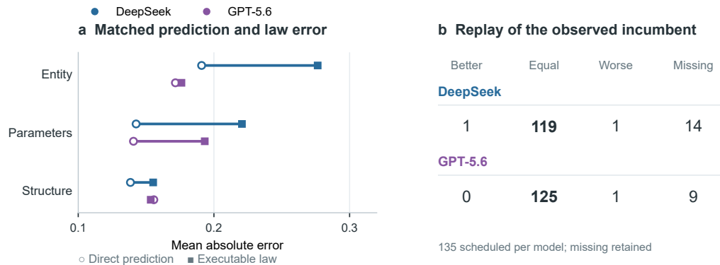
Figure 4: Lower executable-law error coexists with near-zero incumbent gain. a , Hollow circles and filled squares show final-prediction and executable-law MAE on the same law-evaluable cells, grouped by locus and model; connecting lines show compression differences, not uncertainty. The matched denominators are 135 DeepSeek and 129 GPT laws. b , Better/equivalent/worse/unavailable incumbent-replay counts retain all 135 scheduled cells per model, with missing outcomes stated explicitly. These are descriptive configuration contrasts and incumbent replays, not causal artifact effects or unseen-action benefits.
