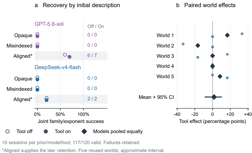
Figure 7: Valid submissions and optional numerics do not ensure structural recovery. a , Joint family/exponent success by prior, model and tool availability; each point retains ten scheduled sessions. All successes are in the aligned-prior stratum, where the correct law was supplied. b , Paired effects in five reused worlds and the equally weighted mean with its prespecified approximate 95% interval. Tool availability is the intervention: GPT used it in 0/30 sessions and DeepSeek in 20/30. Three failures remain in the denominator.
