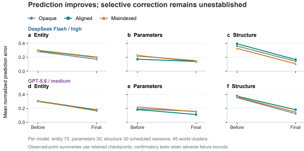
Figure 2: Prediction improves, but the evidence does not establish selective repair of the wrong model. a–c, DeepSeek and d–f, GPT effective pre/final prediction errors by prior and intervention locus; lines connect aggregate observed-point summaries with retained-checkpoint handling. Each model has 135 scheduled sessions in 45 world clusters. Confirmatory tests separately retain adverse failure bounds; all locus criteria are unmet in both models. Initial error limits improvement headroom. DeepSeek first-recipe differences are 45/45, 45/45 and 44/45 matched clusters; this retrospective check has no repeated same-arm baseline.
