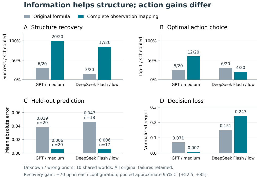
Figure 3: Completing the observation mapping improves structure recovery; action gains differ. a–b , Joint family/exponent recovery and optimal action choice retain 20 scheduled unknown/wrong-prior sessions per configuration and disclosure condition. c , Prediction error uses the available submissions shown by n . d , Failed sessions receive worst normalized regret. All panels show the original attempts, with ten shared worlds; selected failure retries do not replace these outcomes. The two configurations are compared within system, not at equal compute.
