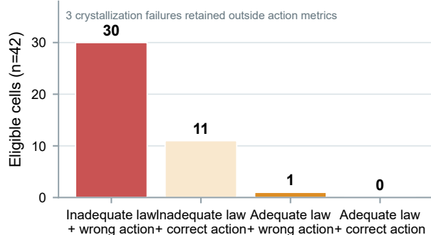
c C Law adequacy did not guarantee action correctness
