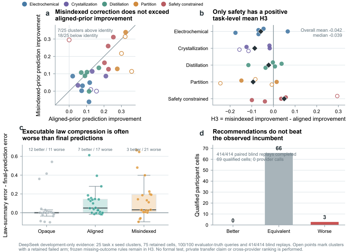
Figure 4. Held-out evaluator confirmation of the five-task DeepSeek development matrix. a , Aligned-prior and misindexed-prior reductions in normalized held-out prediction error for all 25 task-by-world clusters. The identity line marks equal improvement; filled points are complete three-arm clusters and open points retain at least one failed arm under the frozen missing-outcome rule. b , The primary development contrast C_{\text{prior}} by task and seed. Diamonds are task means; positive values favor greater correction in the misindexed arm. c , Executable law-summary error minus final explicit-prediction error for 71 evaluable summaries. Negative values indicate beneficial compression. d , Paired blind replay of the committed recommendation versus the observed incumbent for 69 qualified cells. The evaluator completed 414/414 replays with zero provider calls. All panels are development-only descriptive evidence; no formal test, private transfer claim or cross-provider ranking is performed.
