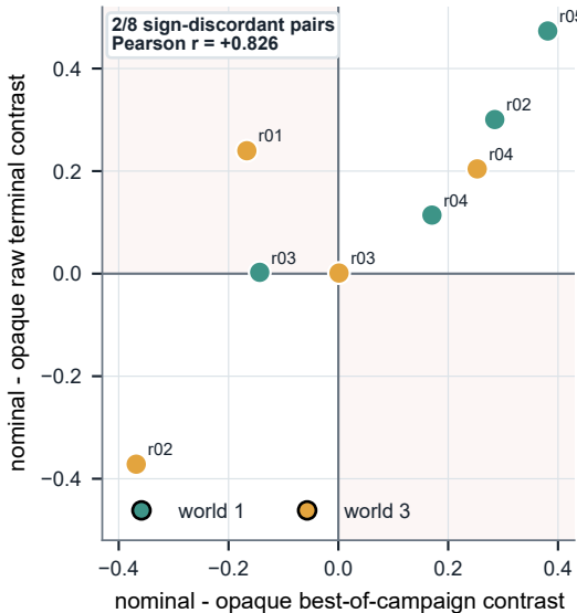
A Best and raw terminal scores can disagree
