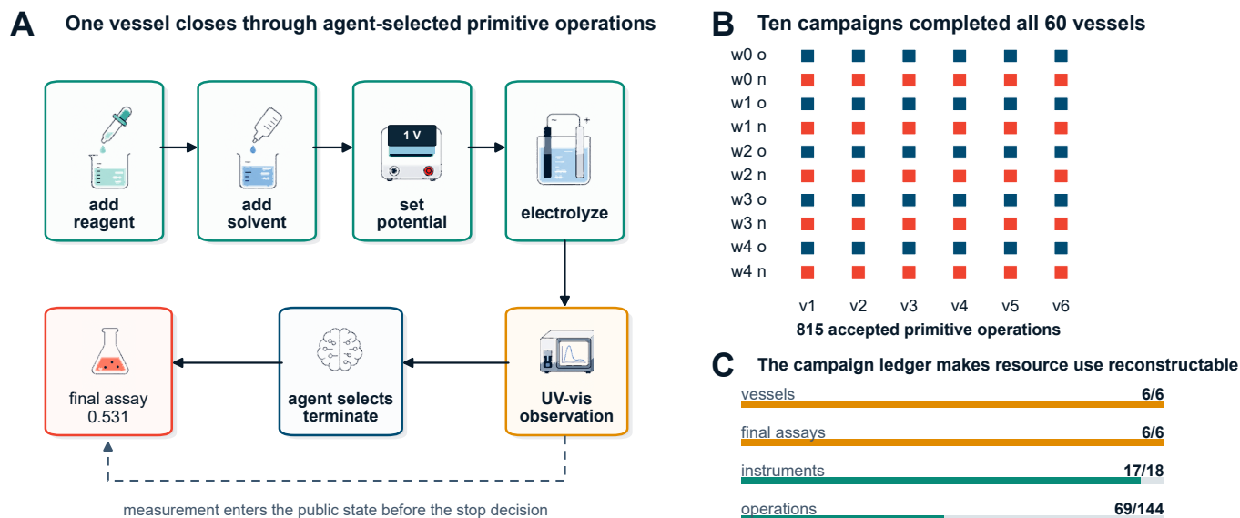
Figure 3. A primitive-control agent closes complete experimental lifecycles. A , One seven-operation vessel in which a UV-visible observation is available before agent-selected termination and explicit final assay. B , All six Codex vessels reached final assay in each of ten world-by-information campaigns; navy denotes opaque codes and coral denotes nominal properties. C , The immutable trajectory reconstructs the campaign resource receipt. The example is descriptive and is not part of the fresh-session replication estimand.
