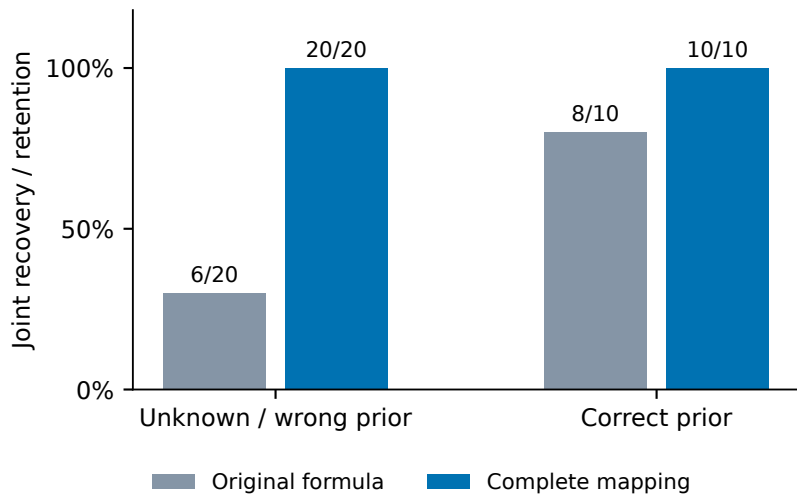
C Held-out prediction
