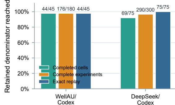
d Execution completeness Failures remain in the denominator
