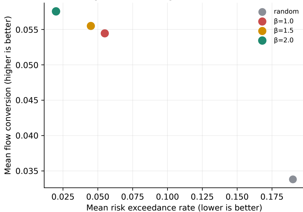
b Lower \beta does not improve the frontier
