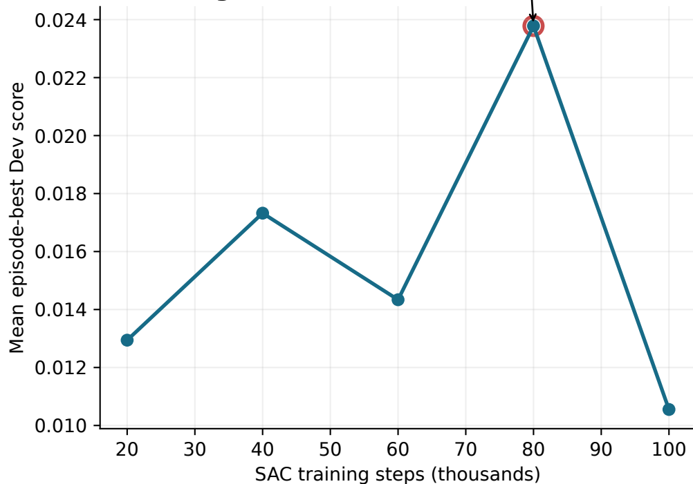
a Training is non-monotonic
