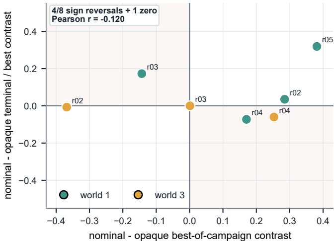
A Best-score direction does not fix terminal retention
