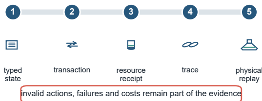
Figure 1. ChemWorld is a controlled apparatus for measuring experimental agency. A , The agent selects a typed action, the executable world changes state, and only the public observation returns to the agent; the transition also writes a resource ledger and immutable trace. B , Physical identity and material information can be matched or intervened on while authority, evidence and resources remain explicit parts of the protocol. C , Typed state, transactions, receipts, traces and physical replay form an auditable spine; invalid actions and failures remain evidence. D , Qualified platform surface and the narrower evidence scope used in this paper.
