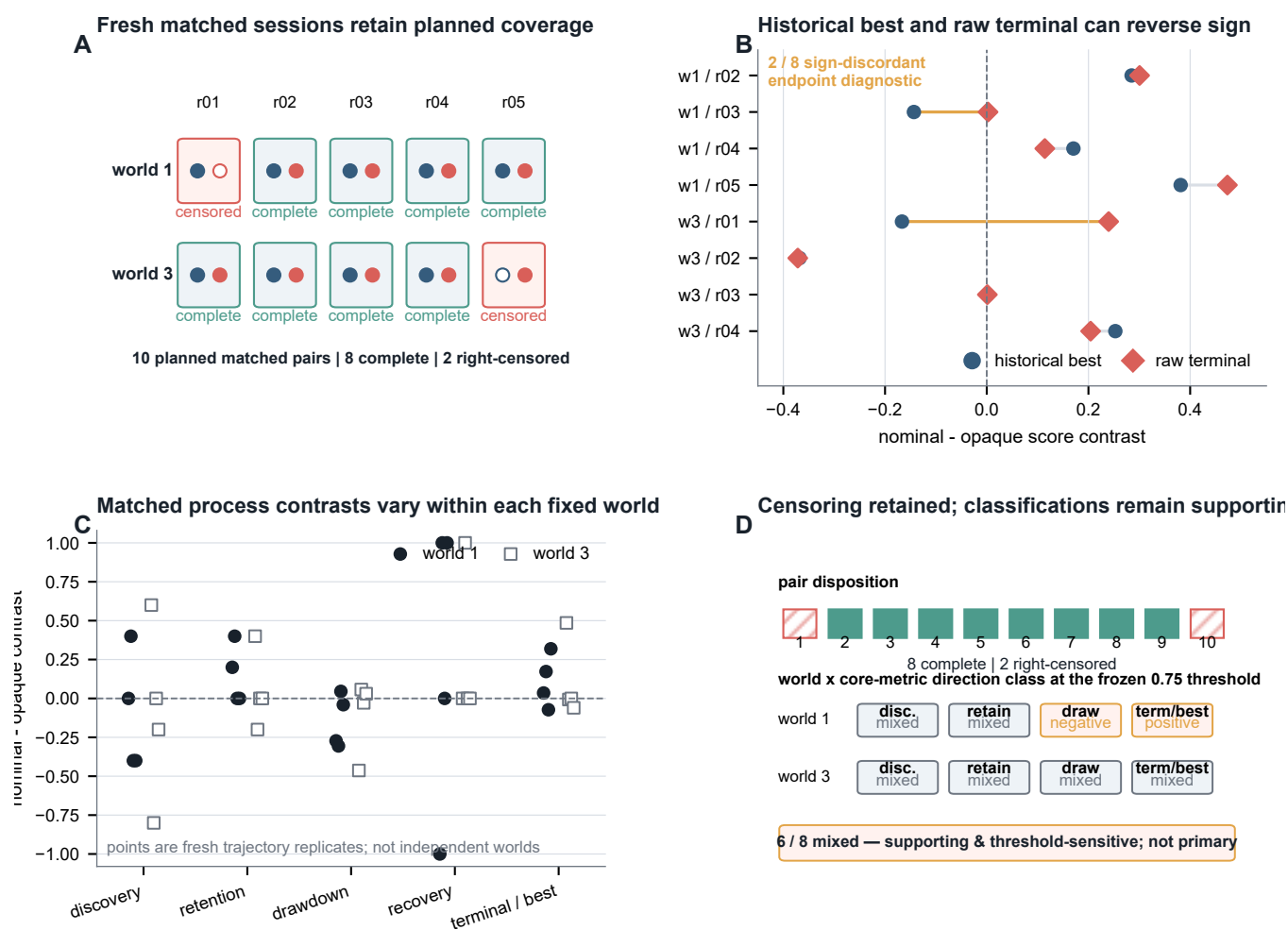
Figure 6 | Fresh trajectories reveal process structure omitted by endpoints. All ten pre-specified trajectory pairs are shown. A , The frozen selected-world design contains eight complete matched pairs and two explicitly right-censored pairs. B , Best-of-campaign and raw terminal contrasts disagree in sign for 2/8 complete pairs; this is the primary endpoint diagnostic. C , Continuous contrasts separately display discovery, retention, drawdown, recovery and relative terminal retention. D , The 6/8 mixed classification is supporting and threshold-sensitive, ranging from two to eight across the frozen sensitivity grid. These deliberately selected worlds describe within-world process variation and are not pooled into a population-level model or information-effect claim.
