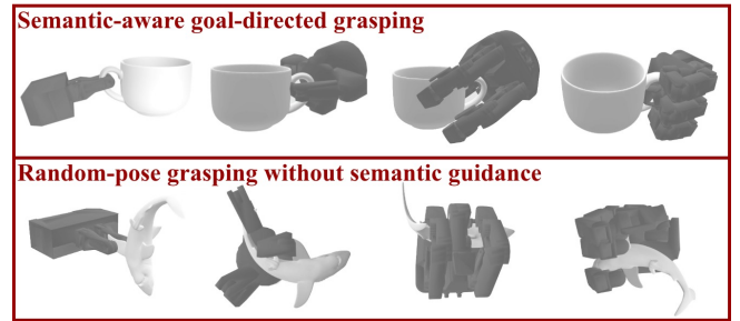
Fig. 4. Qualitative results of synthesized grasps in MuJoCo simulation.
