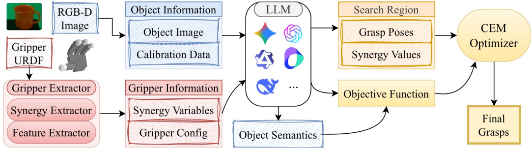
Fig. 2. System architecture for our grasp synthesis. The diagram illustrates the dual object–gripper information streams, LLM-based compilation of search regions and objective functions, and subsequent CEM optimization for final grasp generation.
