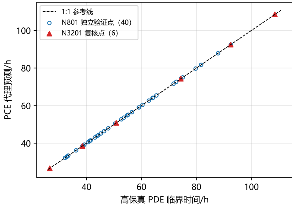
(a) PCE 验证 ( Q^2=0.999999821 , RMSE=0.0069 h)
