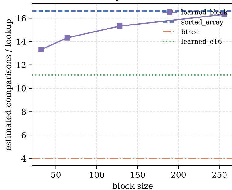
Estimated comparisons vs. block size
