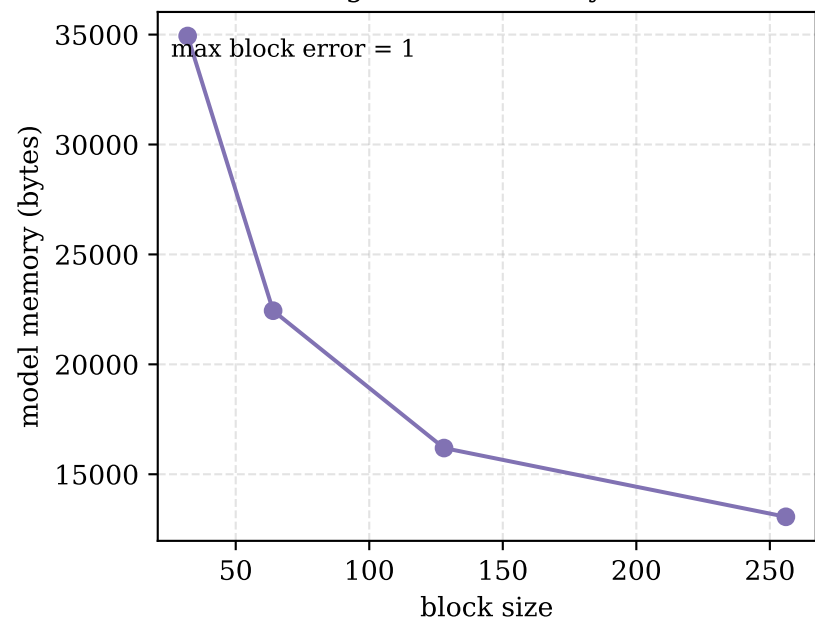
Block-routing: model memory vs. block size
