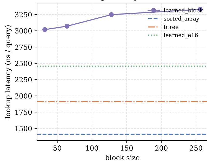
Block-routing: latency vs. block size
