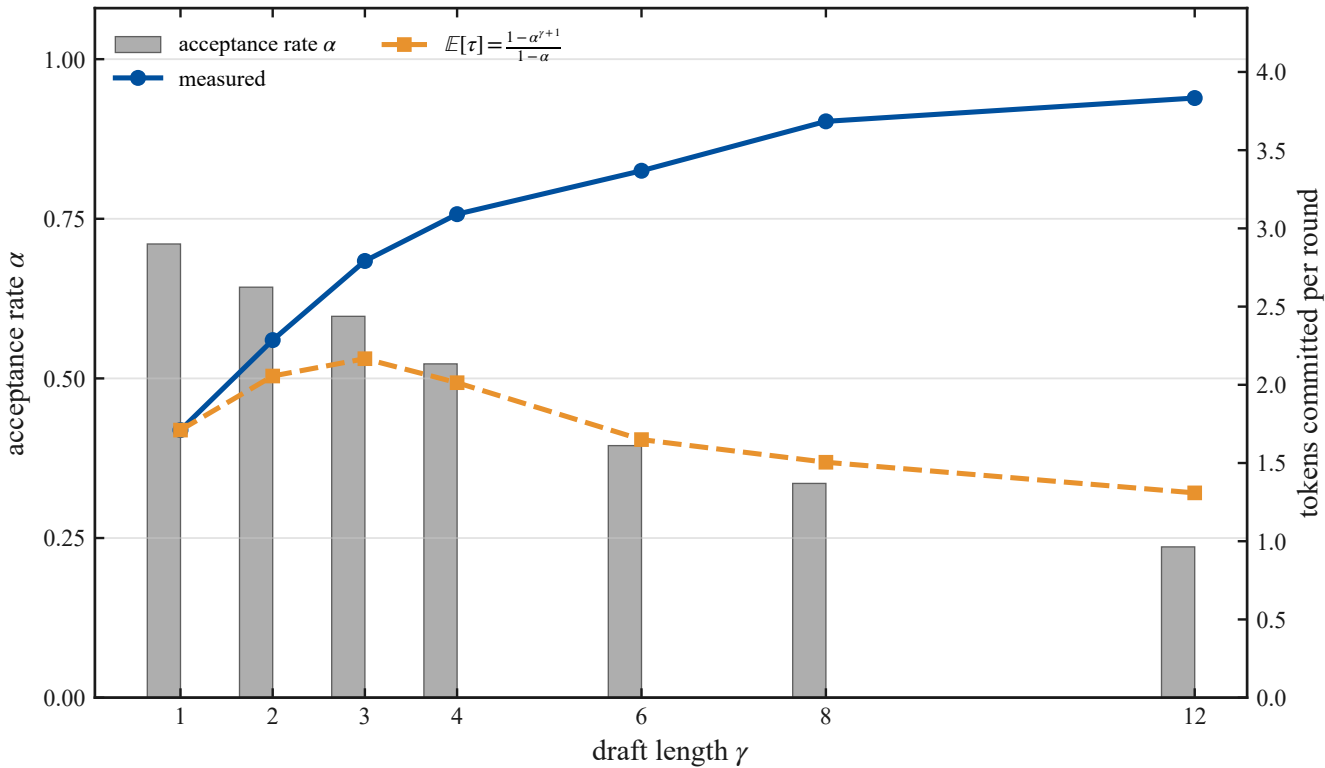
Acceptance rate and committed tokens per round (CPU)
