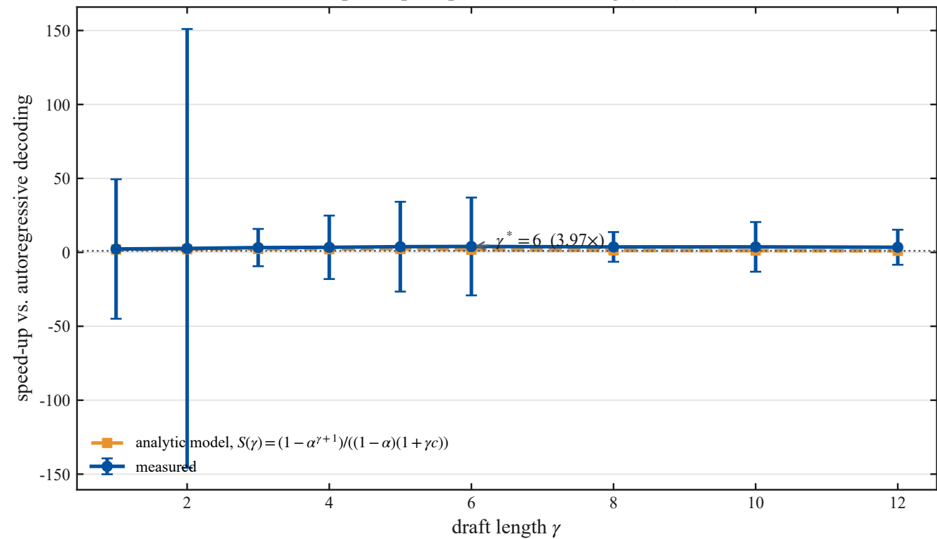
Speed-up of speculative decoding (GPU)
