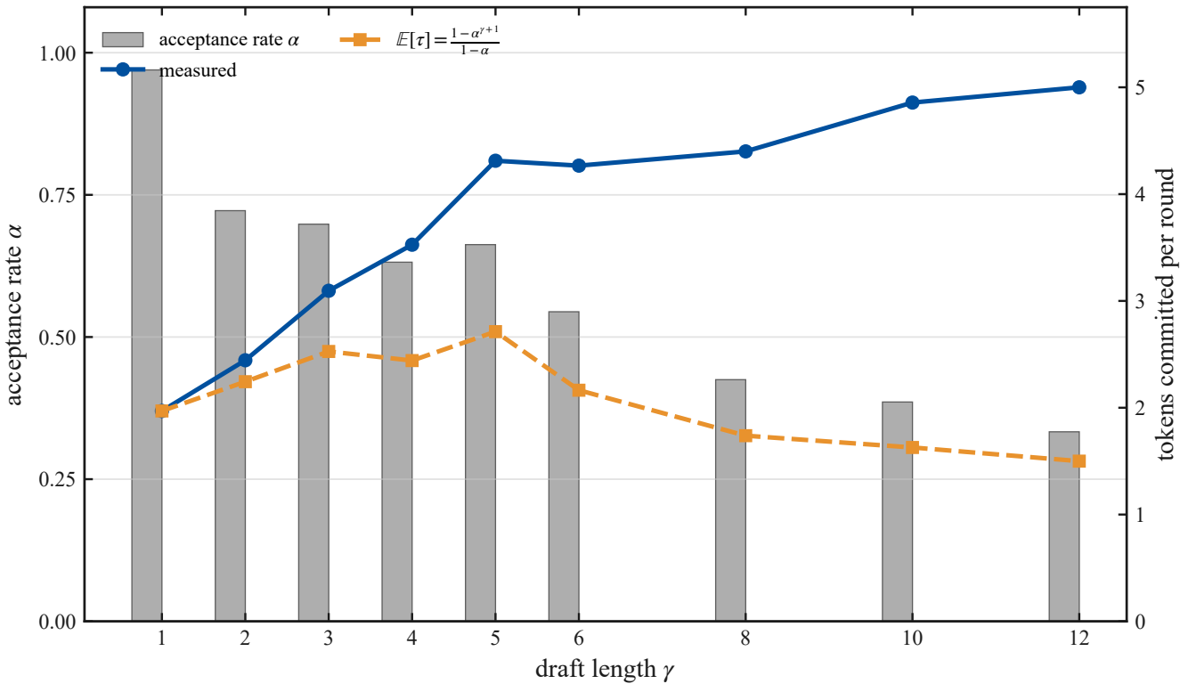
Acceptance rate and committed tokens per round (GPU)
