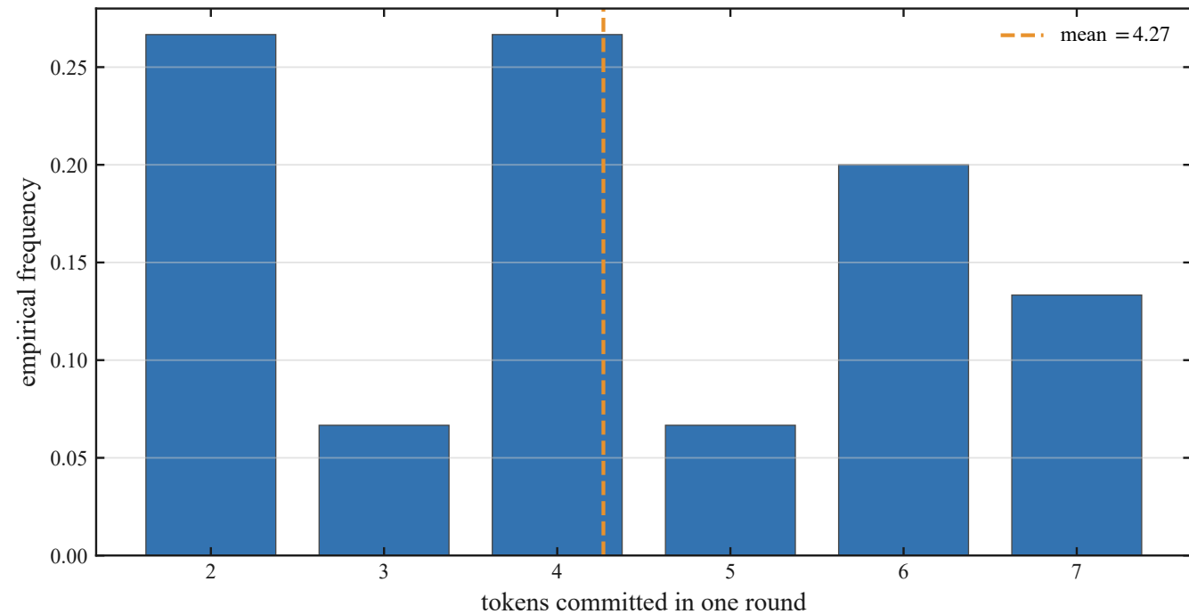
Tokens committed per round at \gamma = 6 (GPU)
