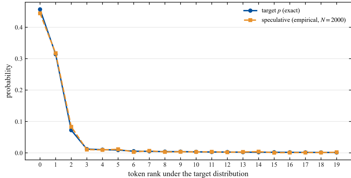
First-token match of the speculative decoder TV = 0.0861, KL = 0.26609, \chi^2 p = 0.754 (GPU)
