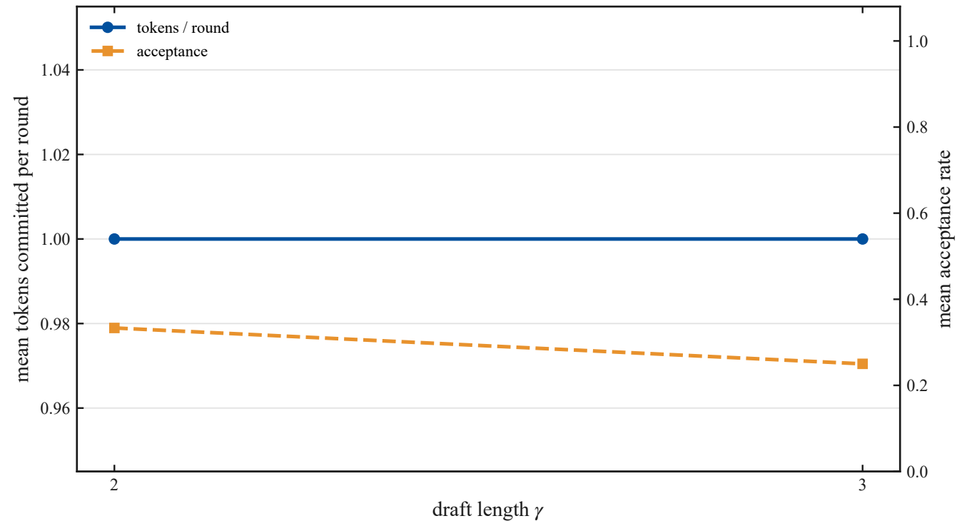
Speculative adaptation vs draft length (CPU)
