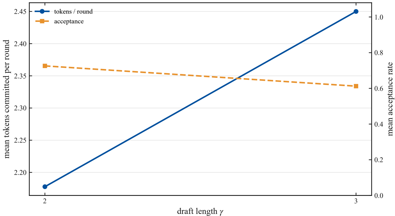
Speculative adaptation vs draft length (GPU)
