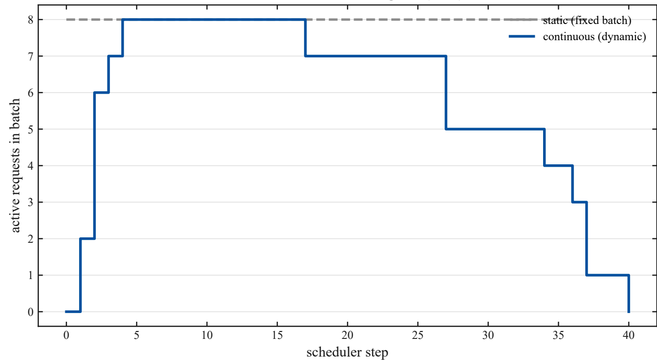
Batch size over the serving run (CPU)
