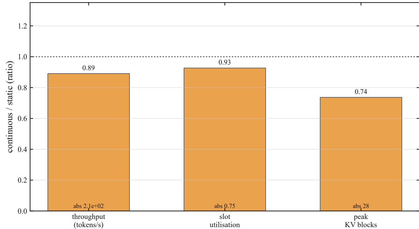
Continuous batching vs static batching (normalised) (CPU)
